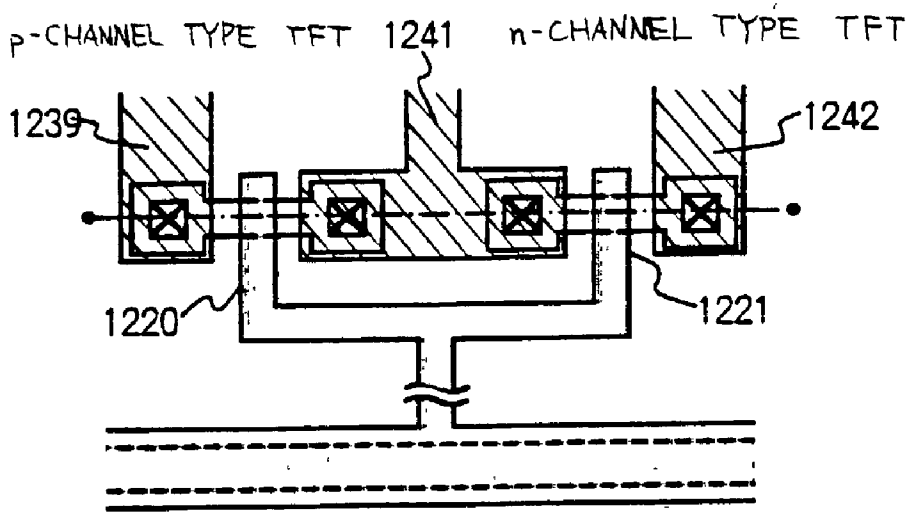
Fig. 10(B) TOP PLAN VIEW OF CMOS CIRCUIT
