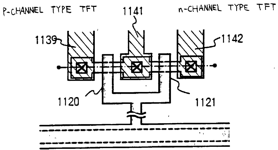
Fig. 10(A) TOP PLAN VIEW OF CMOS CIRCUIT
