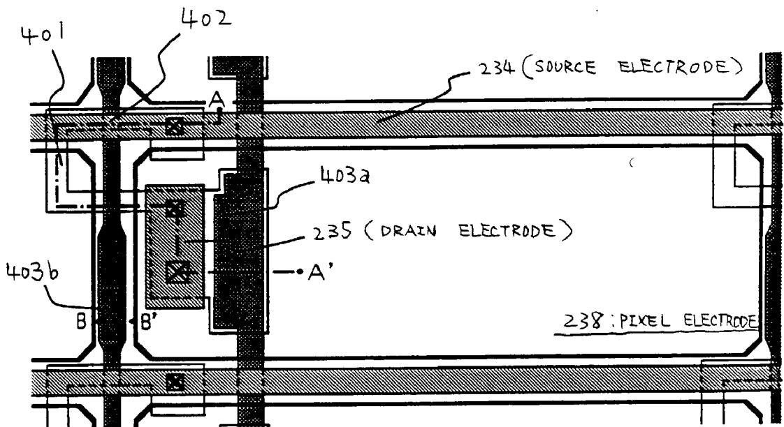
Fig. 5(B) TOP PLAN VIEW SHOWING PIXEL UNIT
