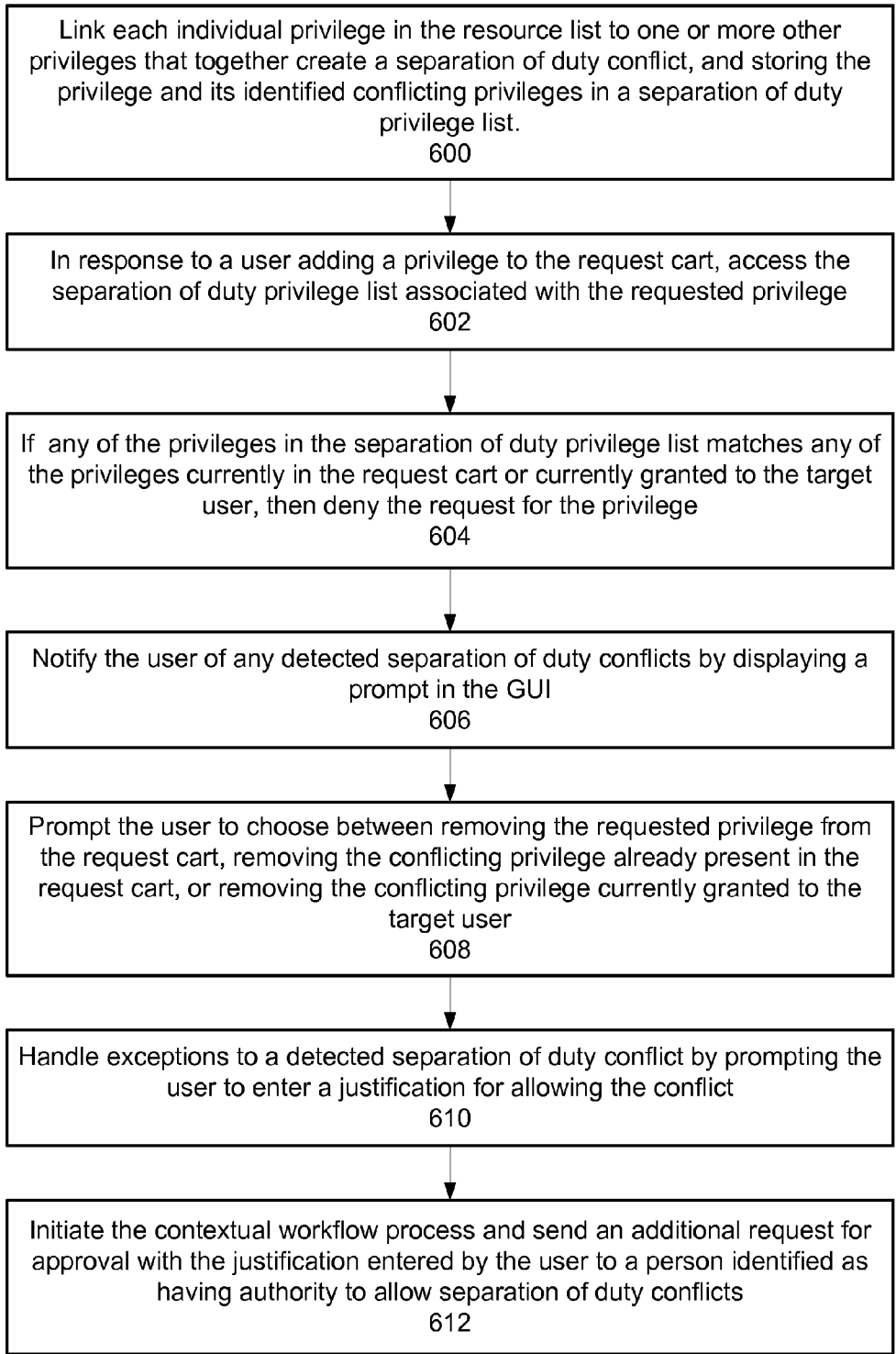
Separation of Duty Detection and Compliance Process
