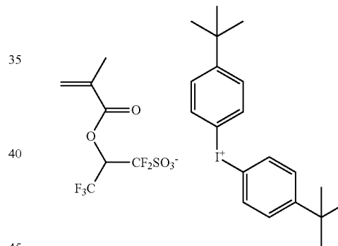
Monomer 2
