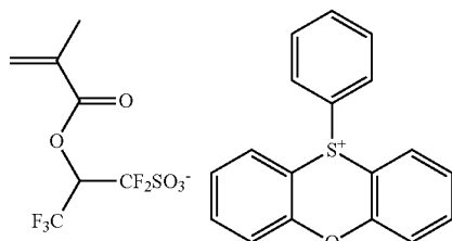
Synthesis Example 37
