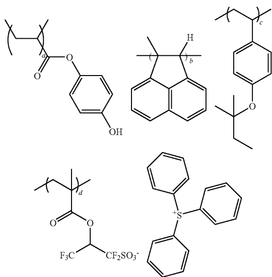
Polymer 1 (C-NMR ratio, a:b:c:d = 51:10:36:3)
