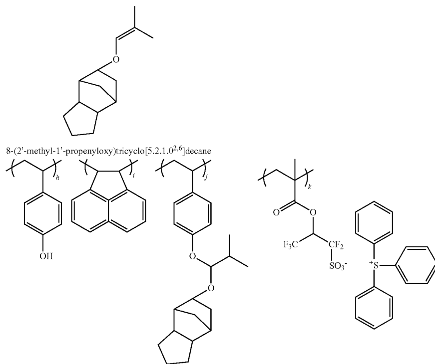
Polymer 39
