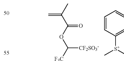
Monomer 3
