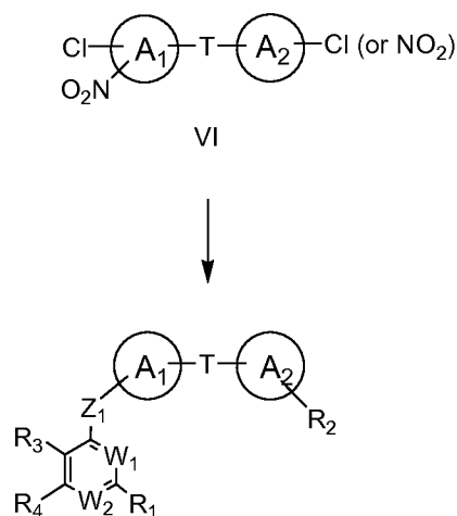
Scheme VII
