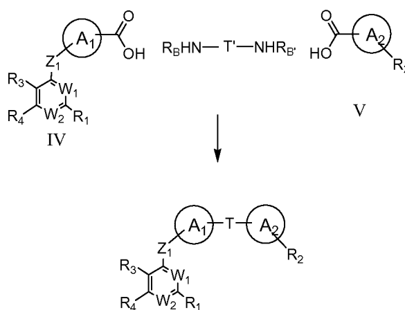
Scheme III
