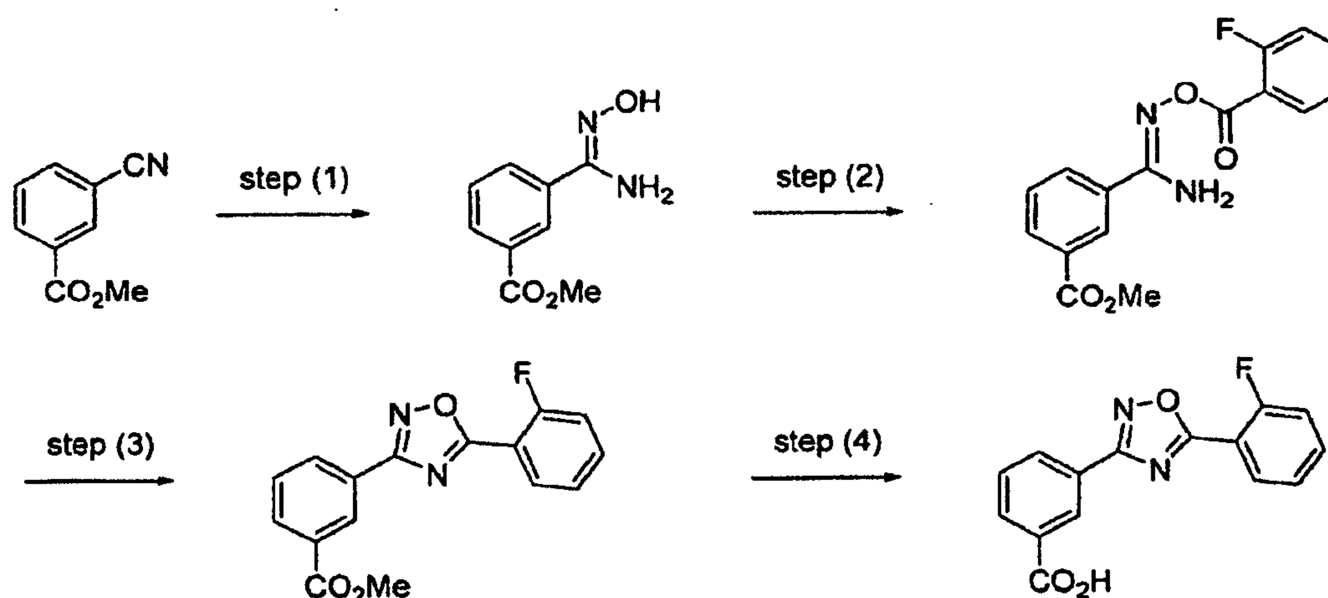
[0119] Scheme 2
