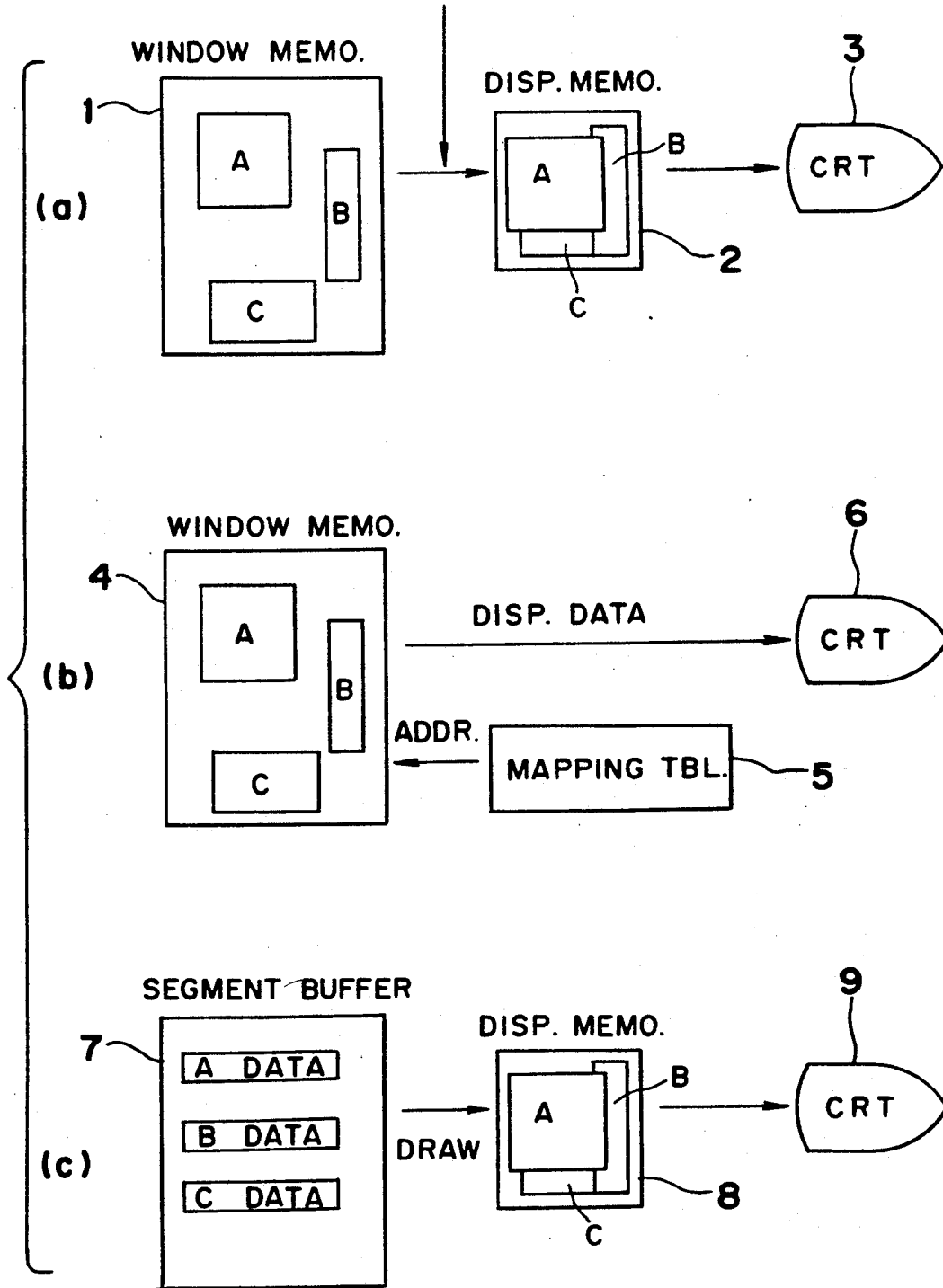
Fig. 5 PRIOR ART
