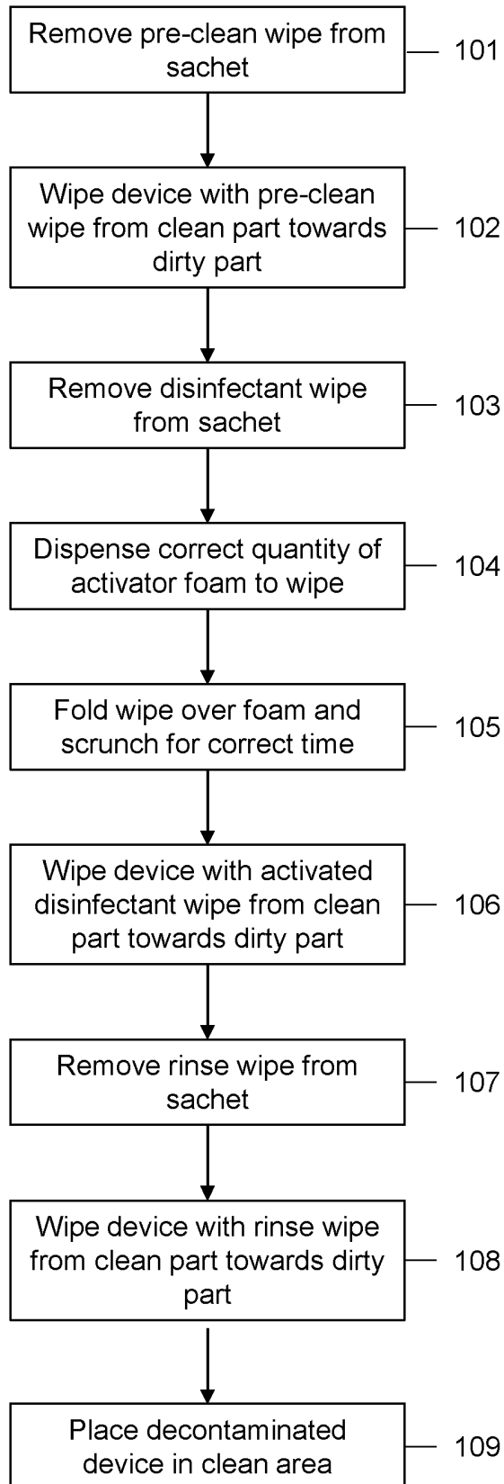
Fig. 2 (PRIOR ART)
