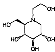
N-hydroxyethyl-deoxynojirimycin
