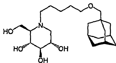
N-(5-adamantane-1-yl-methoxy-pentyl)-deoxynojirimycin
