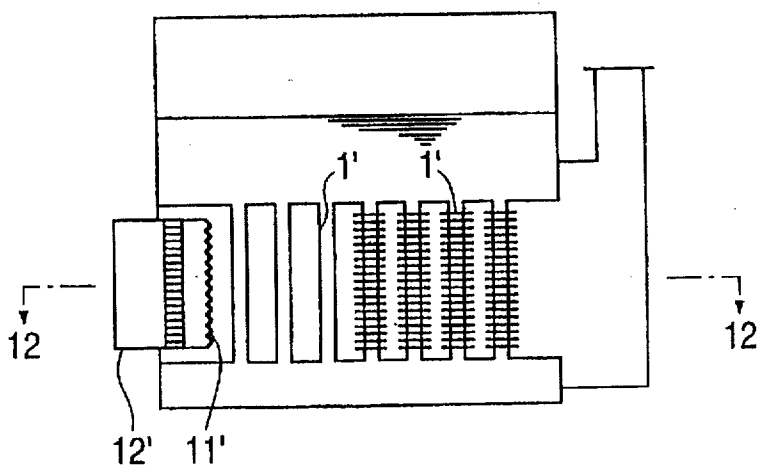
FIG. 11 PRIOR ART
