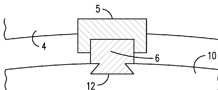
FIG. 2 PRIOR ART
