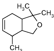
Formula XVIa
