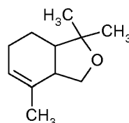
Formula XVIb
