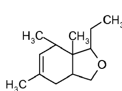
Formula XXIIIa
