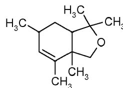
Formula XVIIIb
