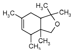
Formula XVIIIa
