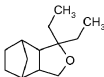
Formula XXI
