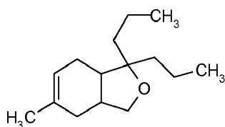
Formula XIXa
