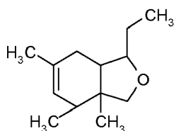
Formula XXIIa
