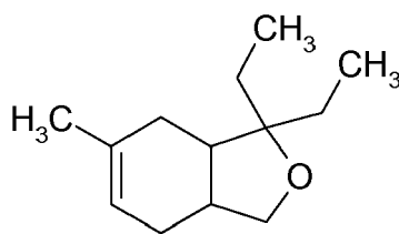
Formula V
