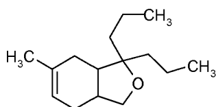
Formula XXa
