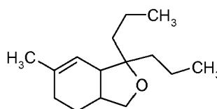
Formula XXb
