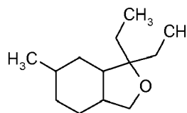
Formula IX
