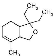
Formula VIb
