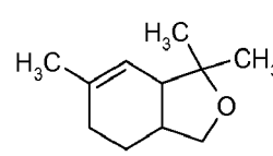
Formula XVb
