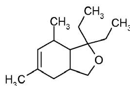
Formula XIa
