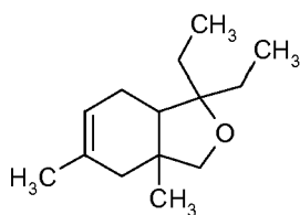
Formula XIIa
