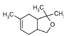
Formula XVa
