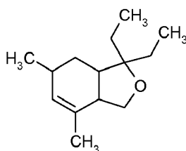
Formula Xb
