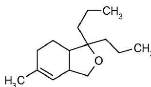
Formula XIXb
