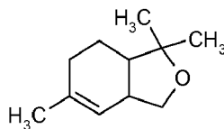
Formula XIVb
