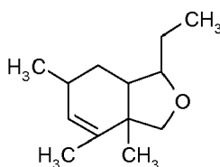
Formula XXIIb
