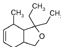
Formula VIIa
