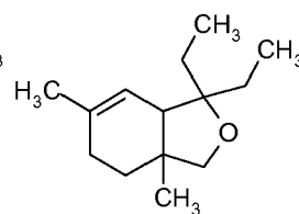
Formula XIIIb
