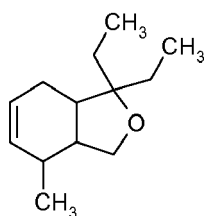
Formula VIa
