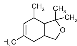
Formula XVIIa
