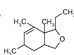
Formula XXIIIb
