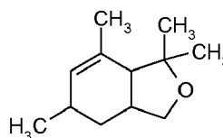
Formula XVIIb
