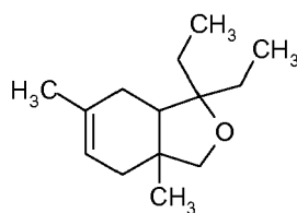
Formula XIIIa
