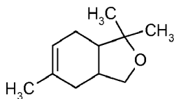
Formula XIVa
