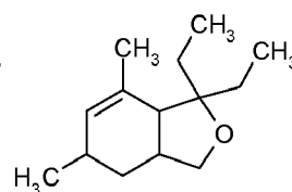
Formula XIb
