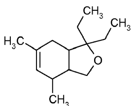
Formula Xa
