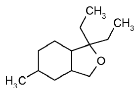
Formula VIII
