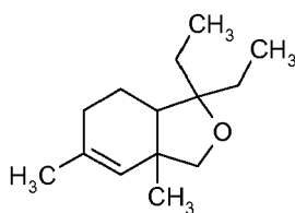
Formula XIIb
