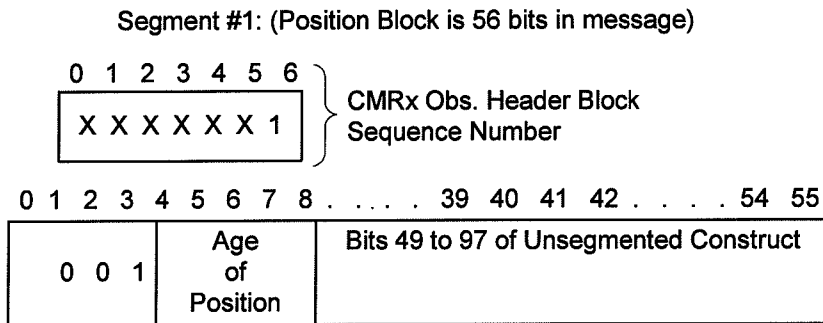
Figure 12. Position Message Sent Over 2 Epochs
