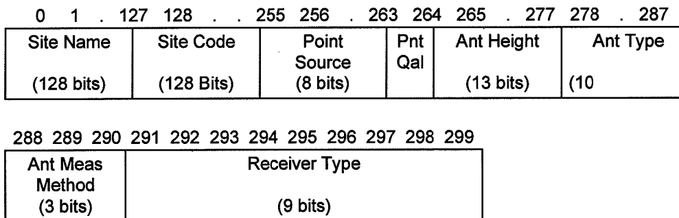
Figure 14. Unsegmented Site Information Construct
