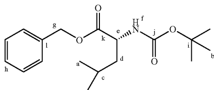
Benzil N-Boc D-leucinate (Compound 46).
