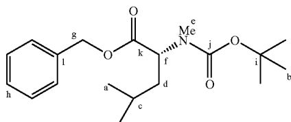
N-Boc N-Methyl benzil D-Leucinate (compound 47).
