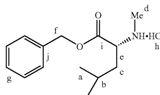
Benzil N-Methyl D-leucinate hydrochloride salt (compound 48).
