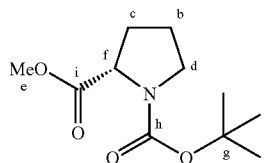
Methyl N-Boc L-Proline (compound 41).
