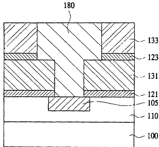
FIG. 1G (PRIOR ART)
