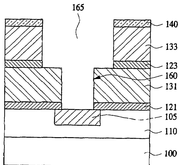
FIG. 1F (PRIOR ART)
