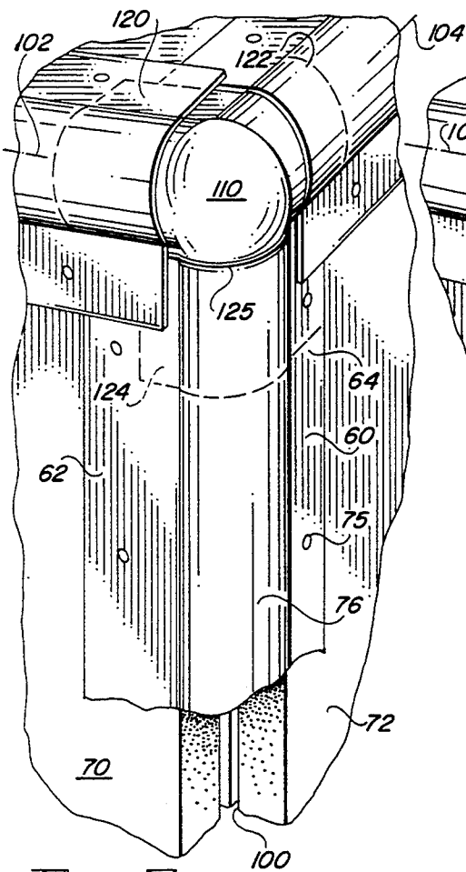
FIG. 7 (PRIOR ART)
