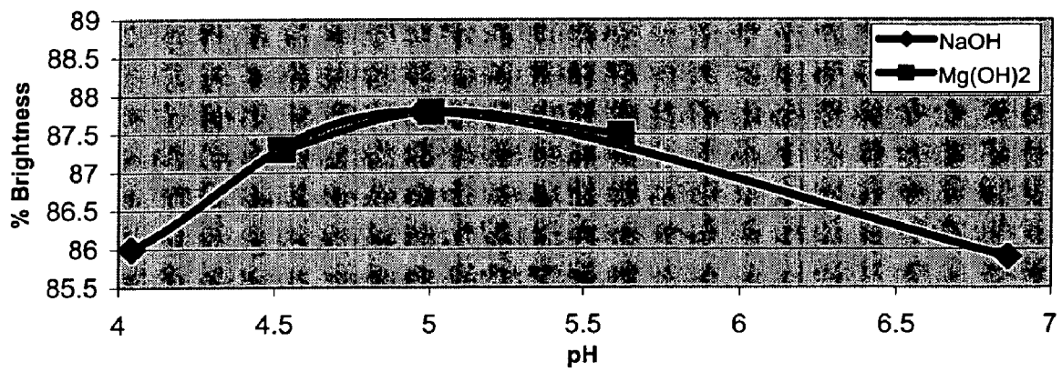
Fig. 7 - Effect of Caustic Source on D1 Brightness
