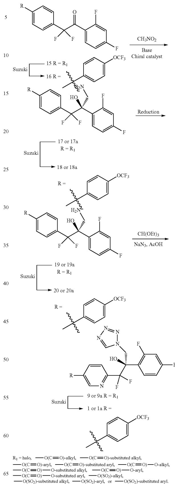
Scheme 7. Asymmetric Henry reaction
