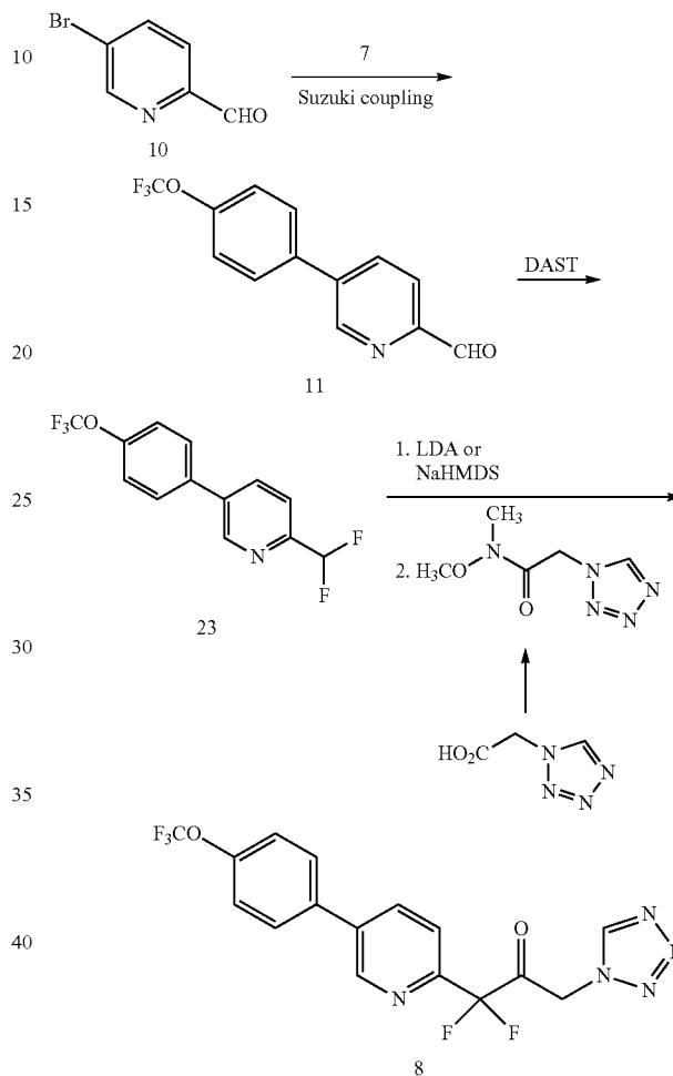
Scheme 4. Alternate synthesis of ketone 8
