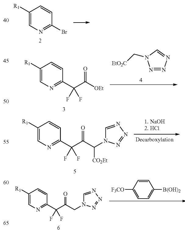
Scheme 2. Synthesis of ketone 8
