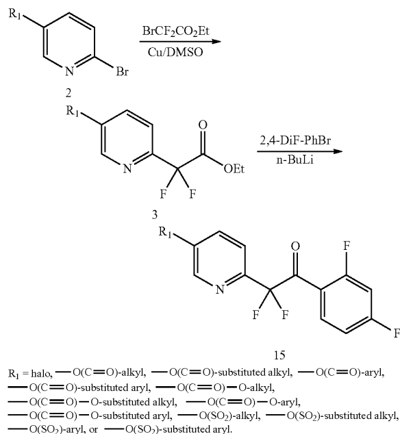
Scheme 6. Synthesis of ketone 15
