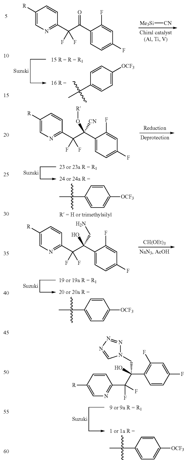
Scheme 9. Asymmetric cyanohydrin strategy
