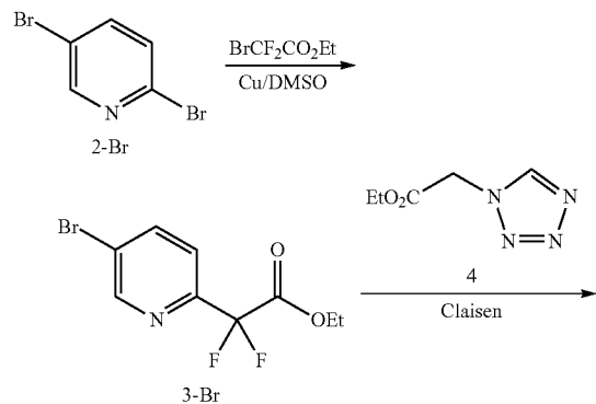
Scheme 1. Synthesis of ketone 8
