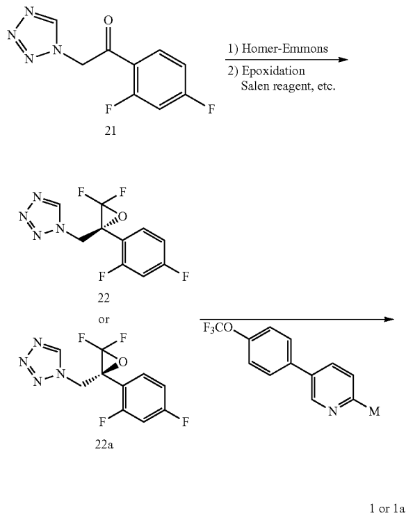
Scheme 8. Enantioselective epoxidation strategy
