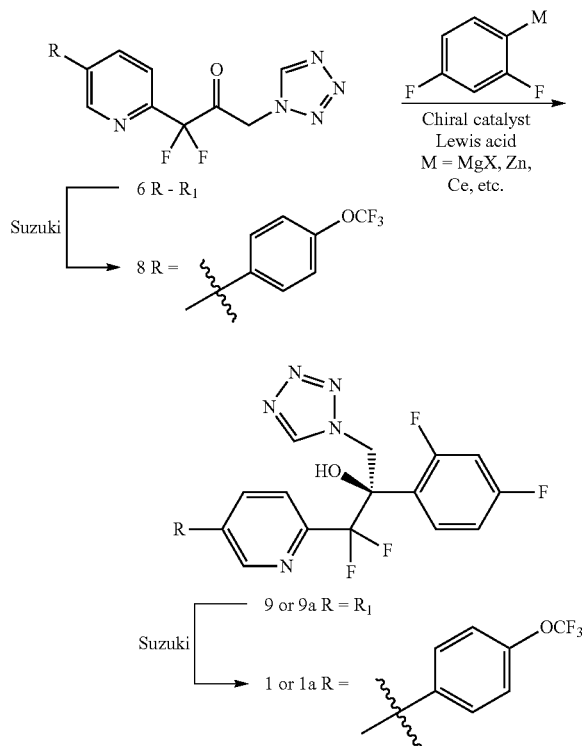
Scheme 3. Synthesis of 1 or 1a
