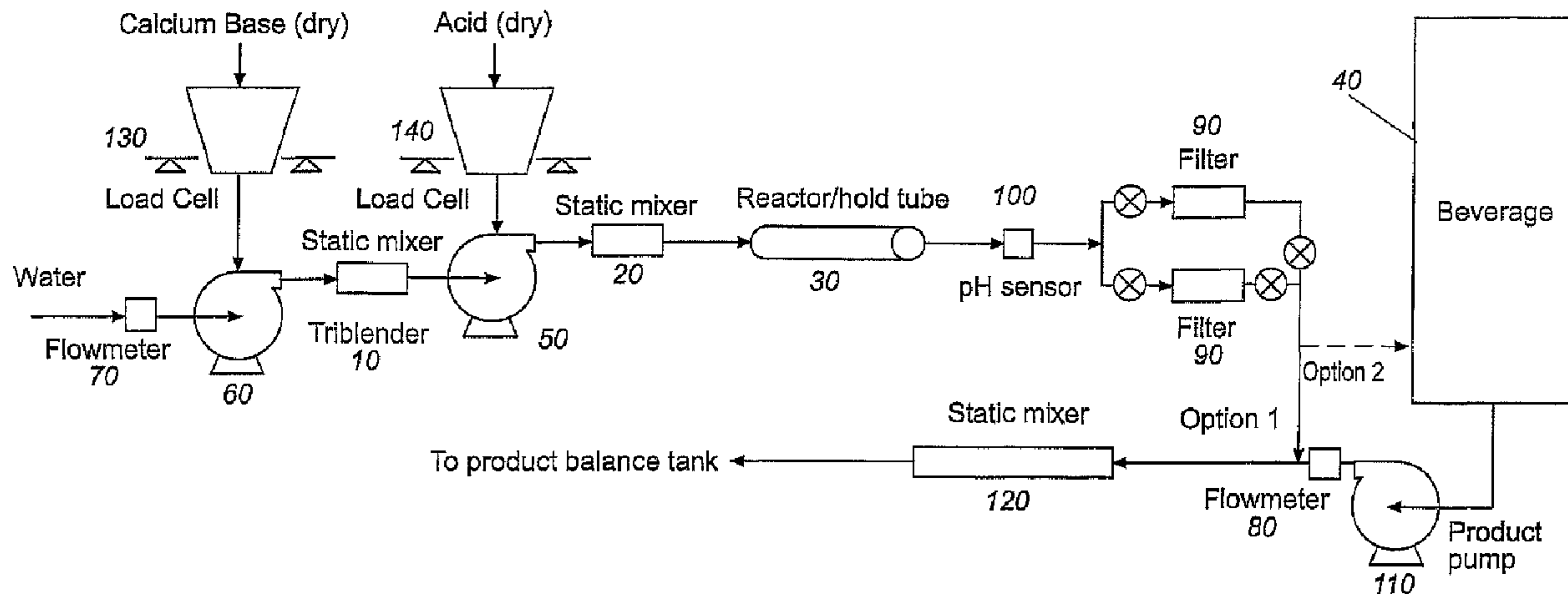
Continuous Blending of Calcium Citrate
