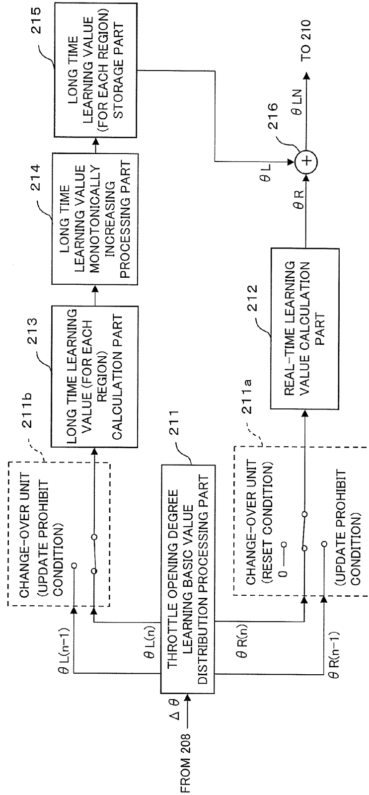
Fig.7 209: THROTTLE OPENING DEGREE LEARNING VALUE CALCULATION PART
