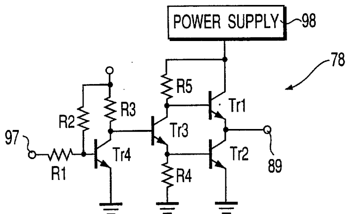
FIG. 22 PRIOR ART
