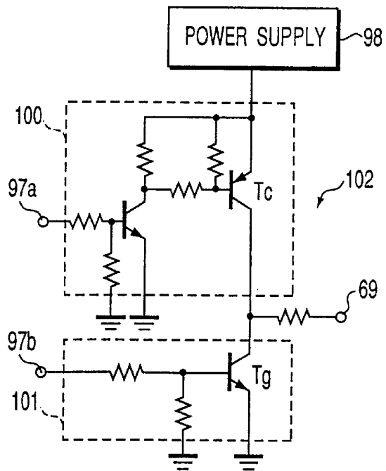
FIG. 24 PRIOR ART
