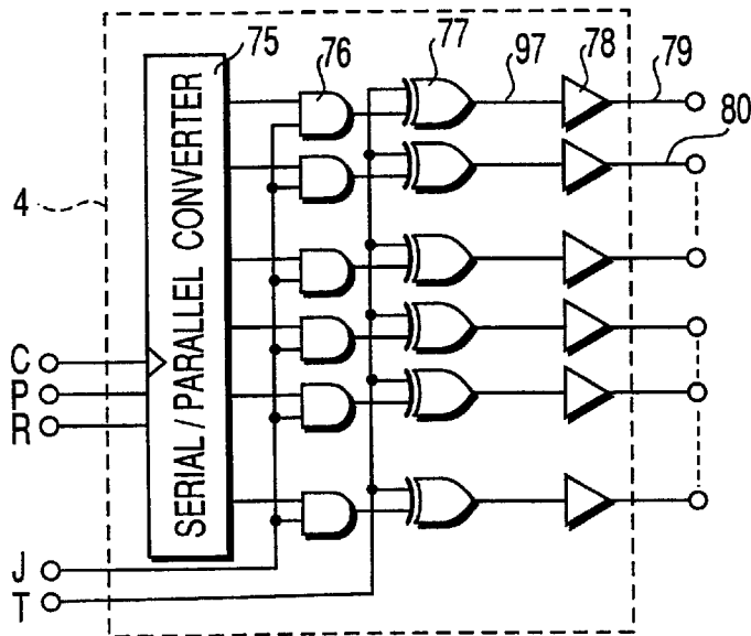
FIG. 21 PRIOR ART
