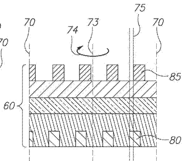
Figure 1F PRIOR ART
