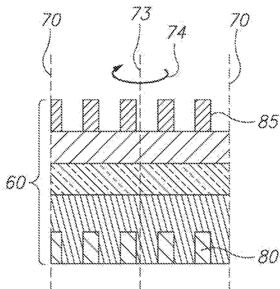
Figure 1H PRIOR ART
