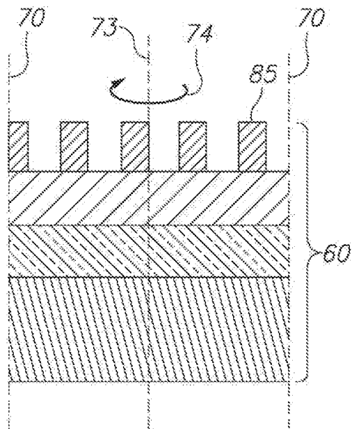
Figure 1D PRIOR ART
