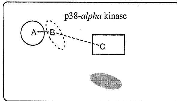
Figure 1. Illustration of the kinase binding domains of known kinase inhibitors
