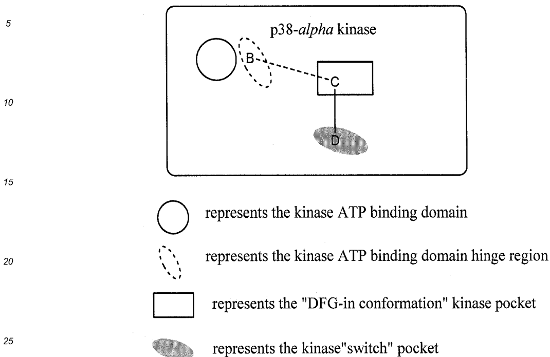
Figure 2. Illustration of the binding modality for compounds of this invention to kinases
