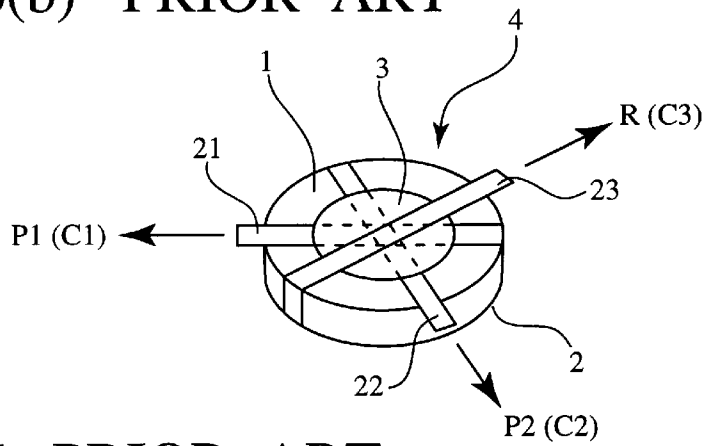
FIG. 7 PRIOR ART
