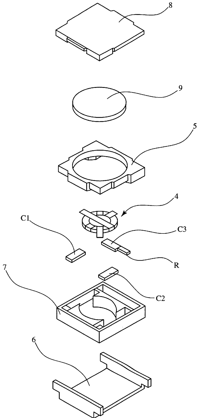
FIG. 5 PRIOR ART
