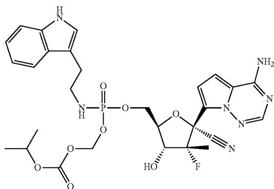
Compound 26
