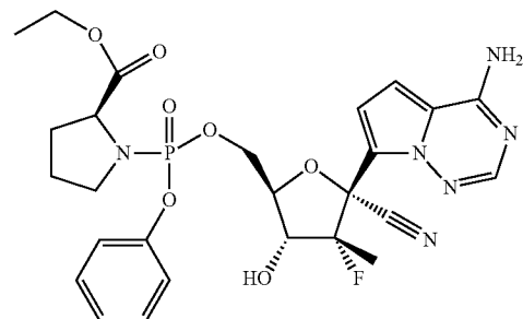
Compound C-5
