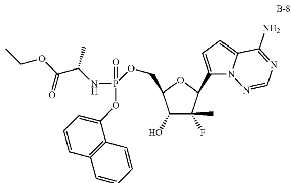
Compound B-8
