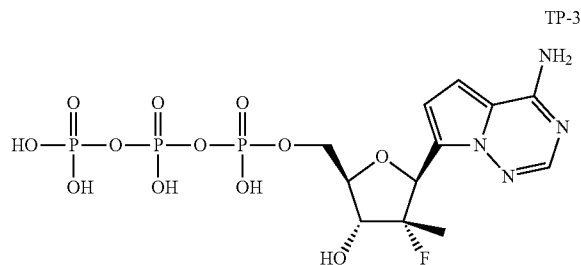
Compound TP-3
