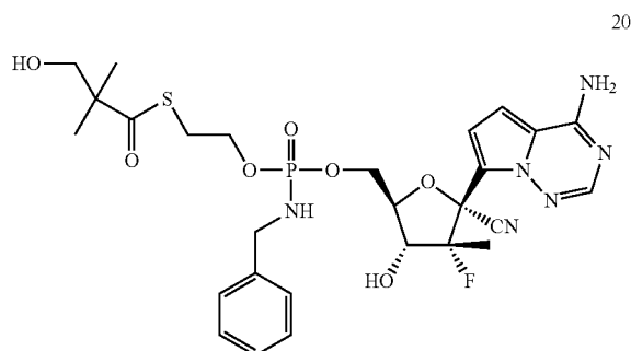
Compound 20
