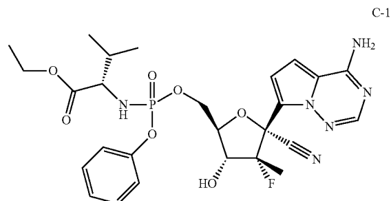
Compound C-1
