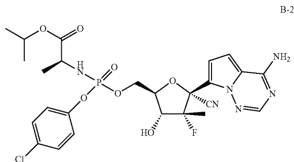
Compound B-2
