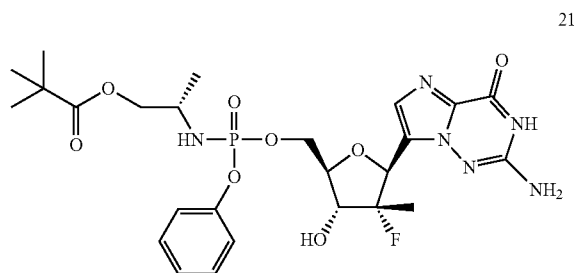
Compound 21
