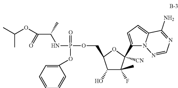
Compound B-3
