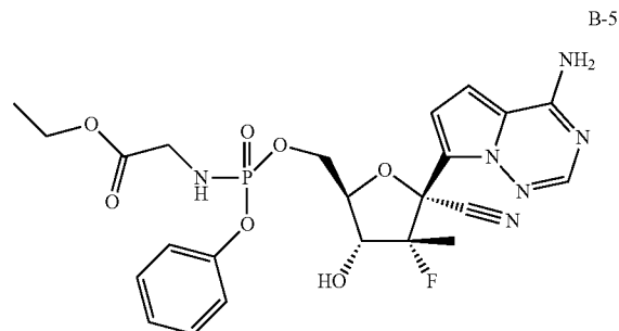
Compound B-5
