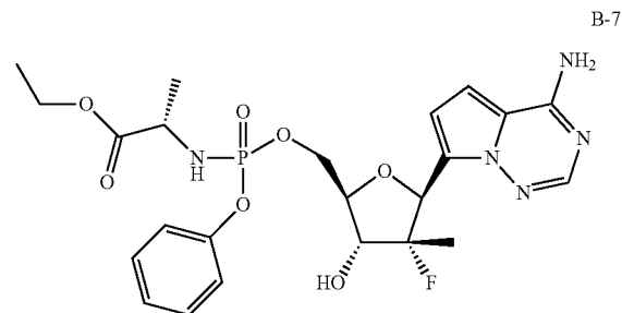
Compound B-7
