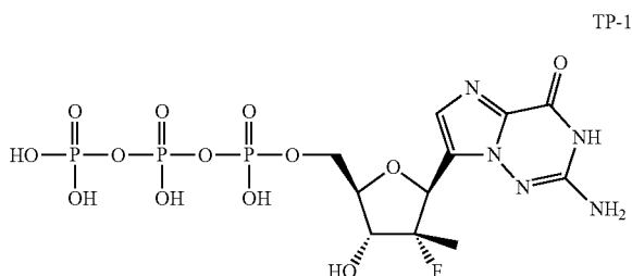
Compound TP-1
