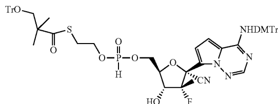
Compound 17
