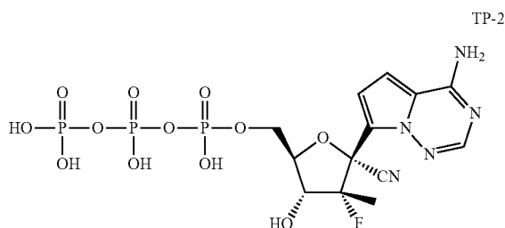
Compound TP-2
