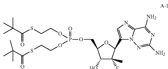
Compound A-1
