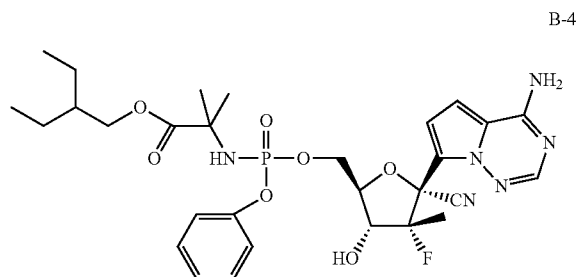
Compound B-4
