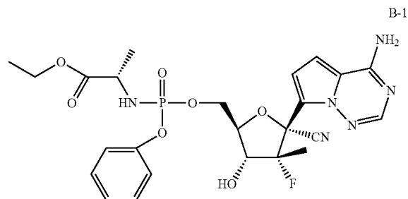
Compound B-1
