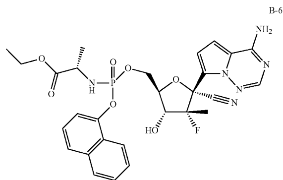
Compound B-6
