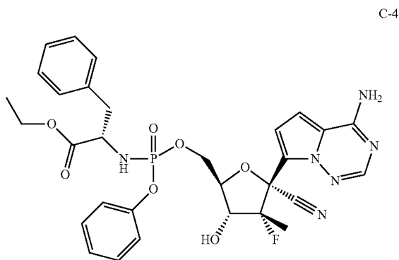
Compound C-4
