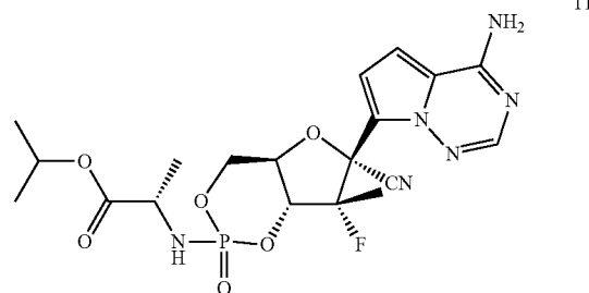
Compound 11
