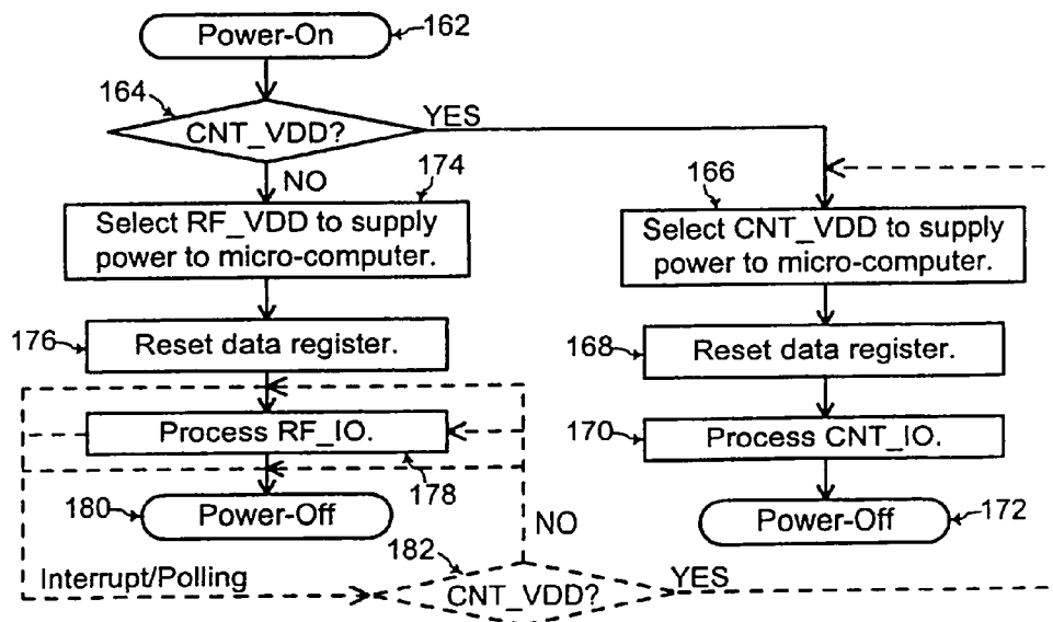
FIG. 6 (Prior Art)
