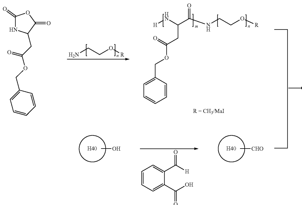
Scheme 1. A synthetic scheme of multi-arm star block copolymer H40-P(Asp-AED-ICA)-PEG-OCH 3 /Cy5/GE11.
