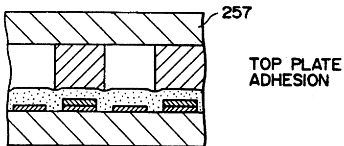
FIG. 2(q) PRIOR ART
