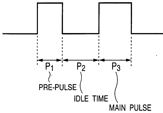
DOUBLE-PULSE DRIVING IN CONVENTIONAL PRINTHEAD
