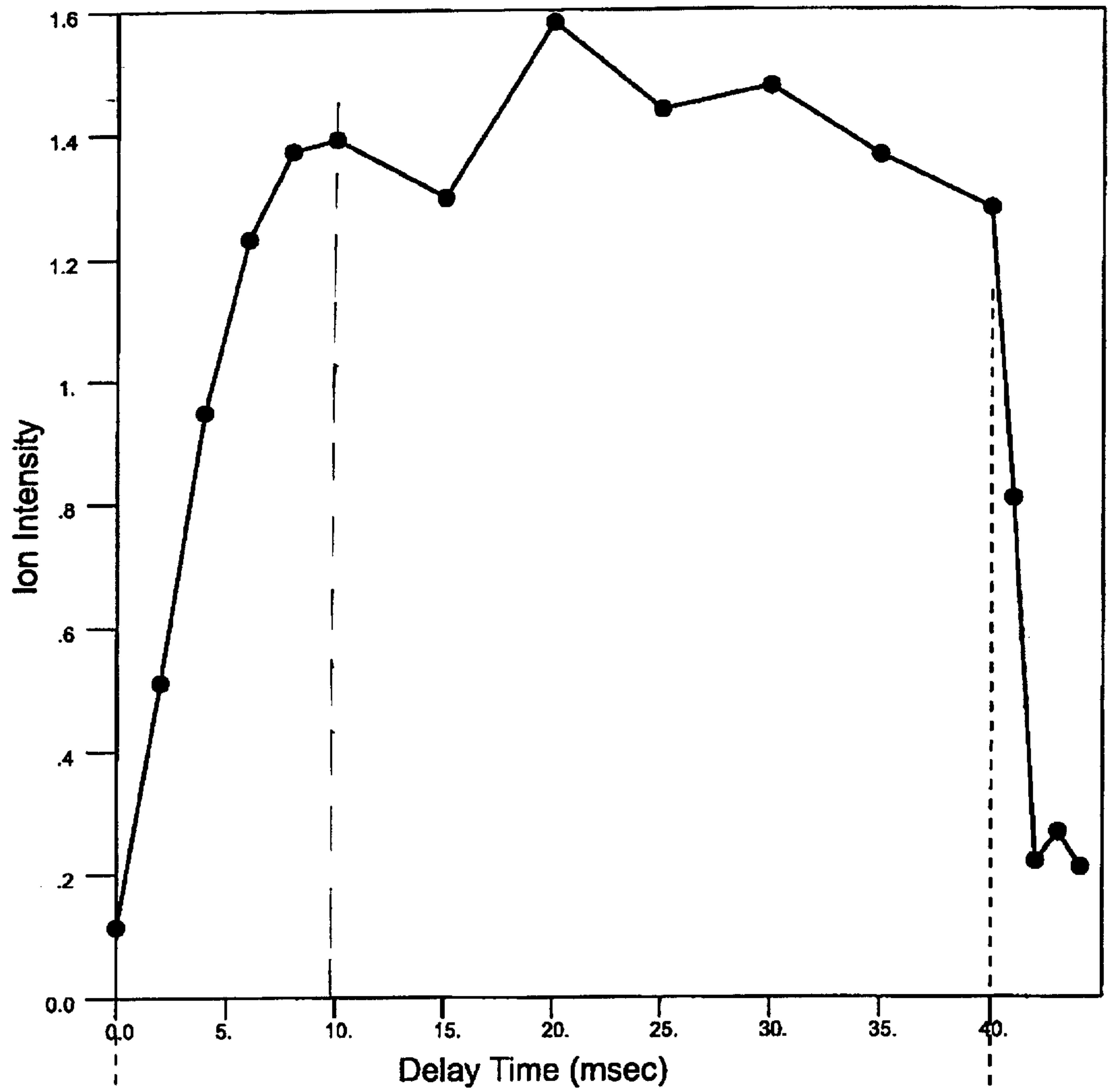
Response Time of Interface, Octopole, and TOF System
