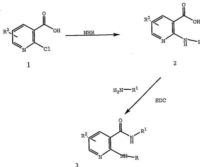
Scheme 1
