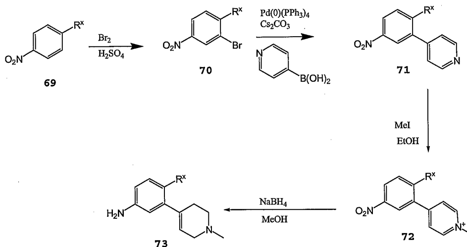
Scheme 20
