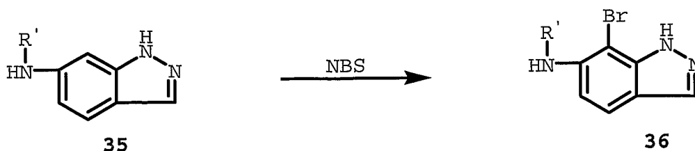
Scheme 12
