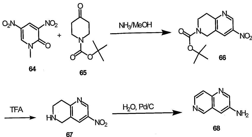
Scheme 19
