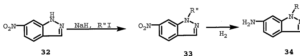
Scheme 11
