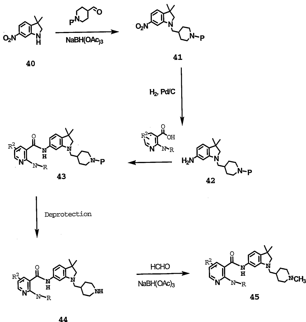
Scheme 14
