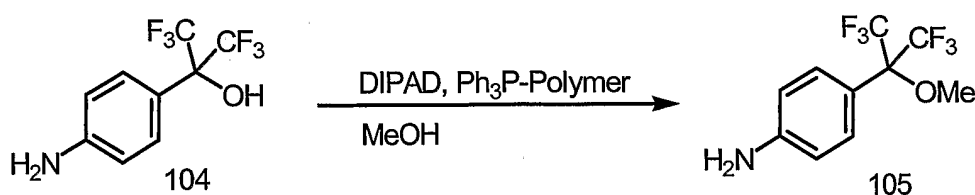
Scheme 27
