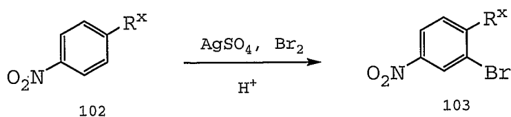
Scheme 26
