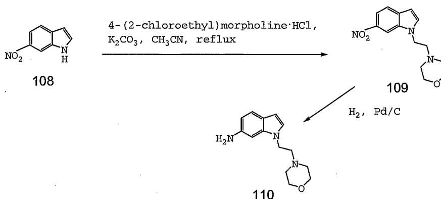
Scheme 29
