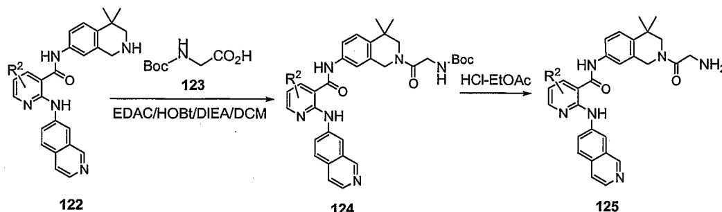
Scheme 33
