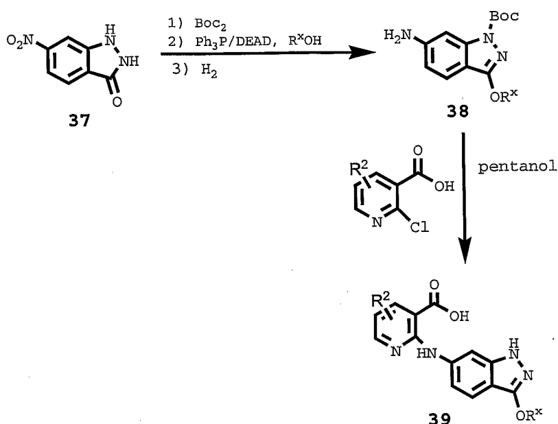
Scheme 13
