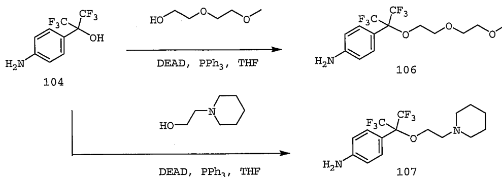
Scheme 28
