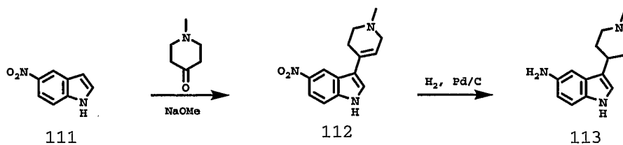
Scheme 30
