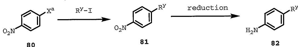
Scheme 22
