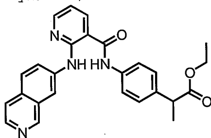
52 2(R,S)-(4-{[2- (Isoquinolin-7-ylamino)- pyridine-3-carbonyl]- amino}-phenyl)-propionic acid ethyl ester
