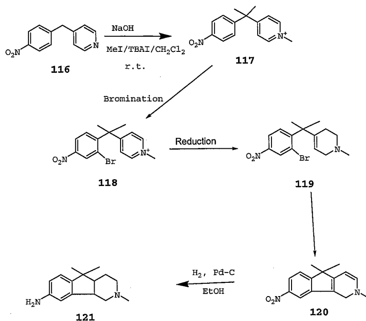
Scheme 32
