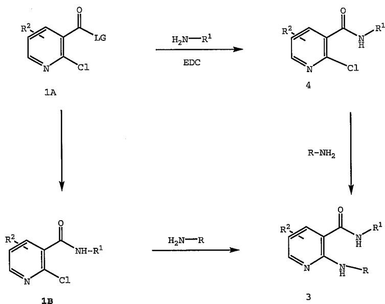
Scheme 2
