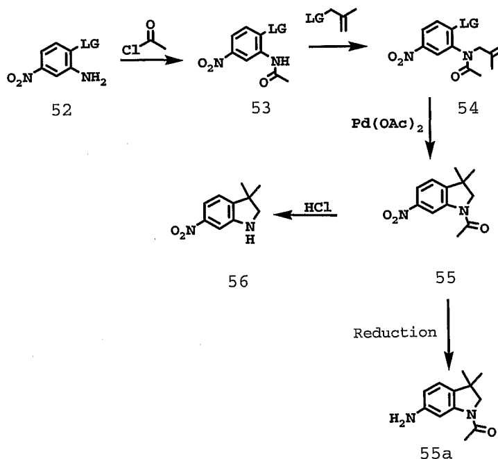
Scheme 16
