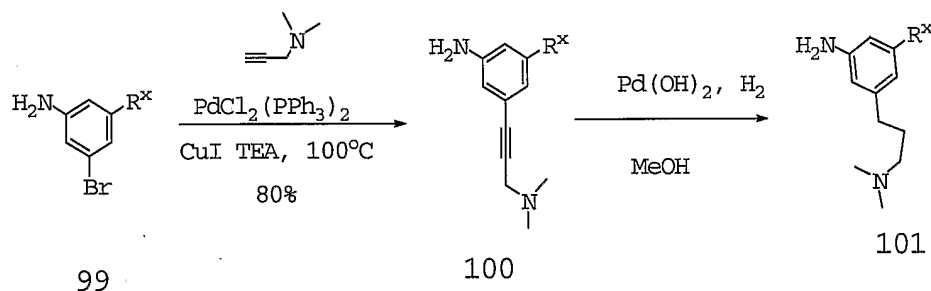
Scheme 25
