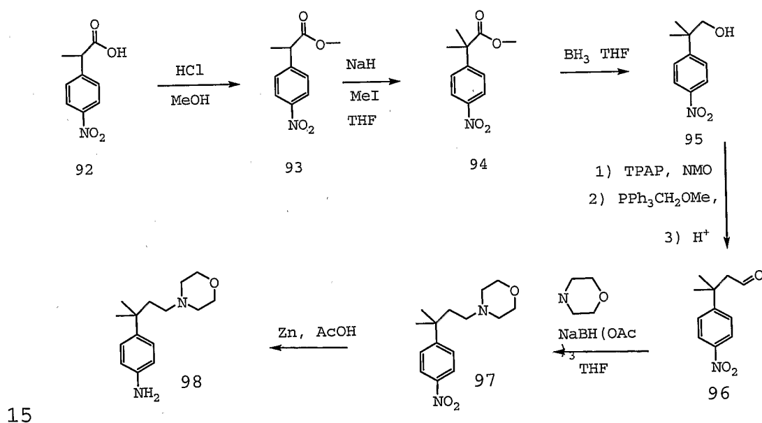
Scheme 24
