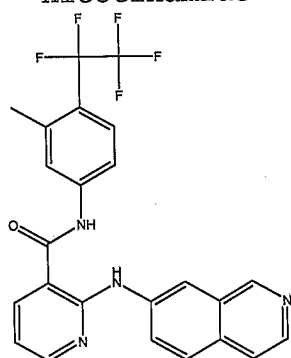
2-(Isoquinolin-7- ylamino)-N-(3-methyl-4- pentafluoroethyl- phenyl)-nicotinamide
