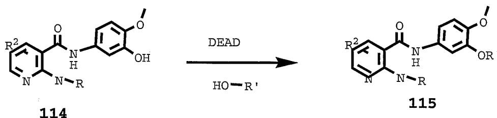
Scheme 31
