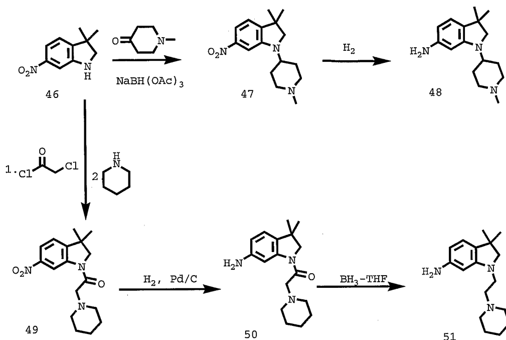
Scheme 15
