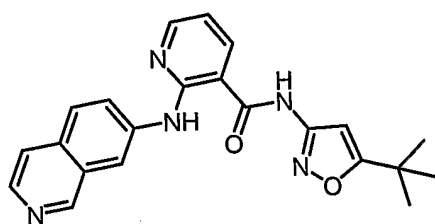
15 N-(5-tert-Butyl- isoxazol-3-yl)-2- (isoquinolin-7-ylamino)- nicotinamide
