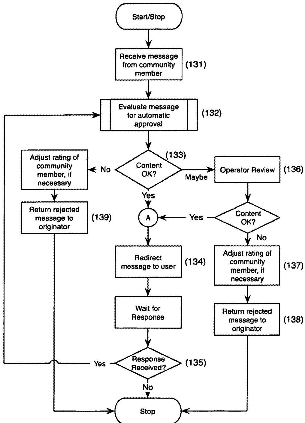
Fig 13. Transport Community Proxy Message Service
