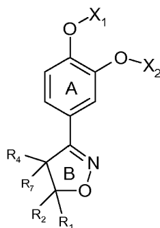
Formula Ib
