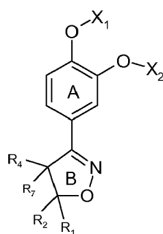
Formula Ib
