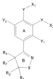
FORMULA Ia
