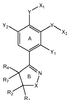
FORMULA Ia
