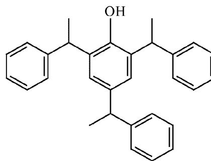
Tristyrylphenol
