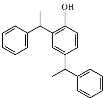
Distyrylphenol
