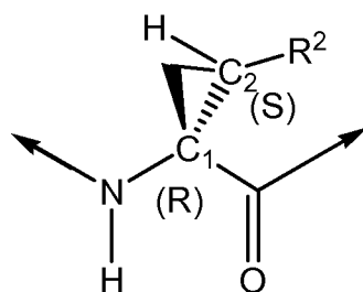
(1R, 2S) R 2 is syn to carbonyl
