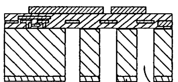
BACKSIDE ETCH 116 114
