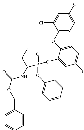
Synthesis of compound 3
