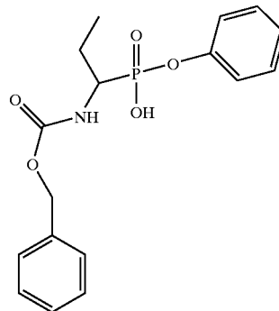
Synthesis of compound 2
