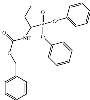
Synthesis of compound 1
