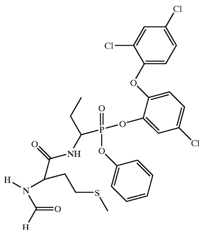
Synthesis of compound 4
