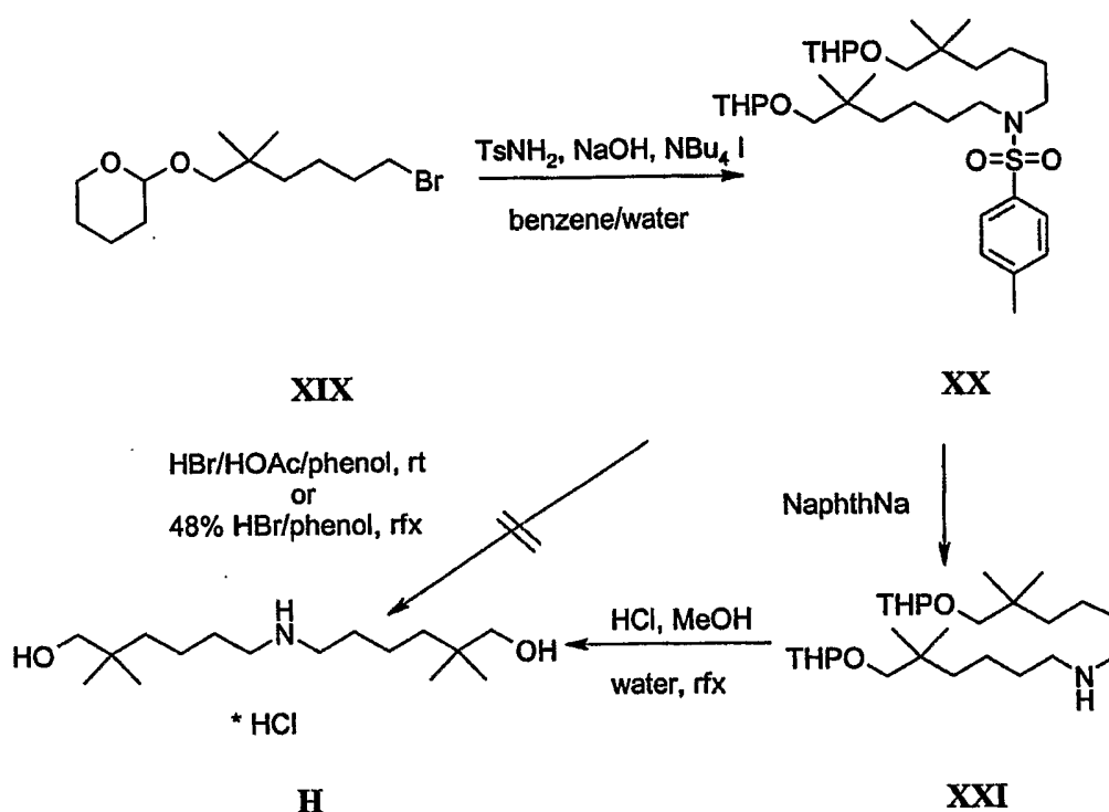
Scheme 6: Synthesis of 6-(5,5-dimethyl-6-hydroxy-hexylamino)-2,2-dimethyl-hexan-1-ol hydrochloride ( H )
