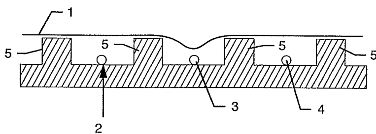
FIG. 1 PRIOR ART
