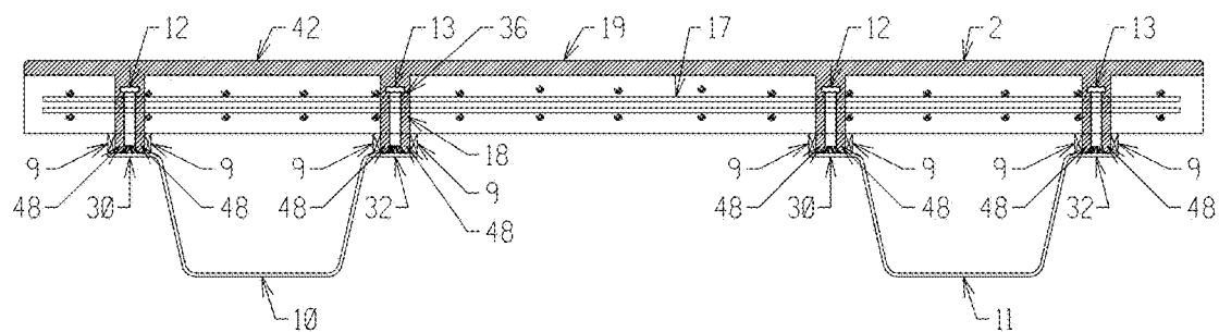
SECTION B-B FIGURE 6A
