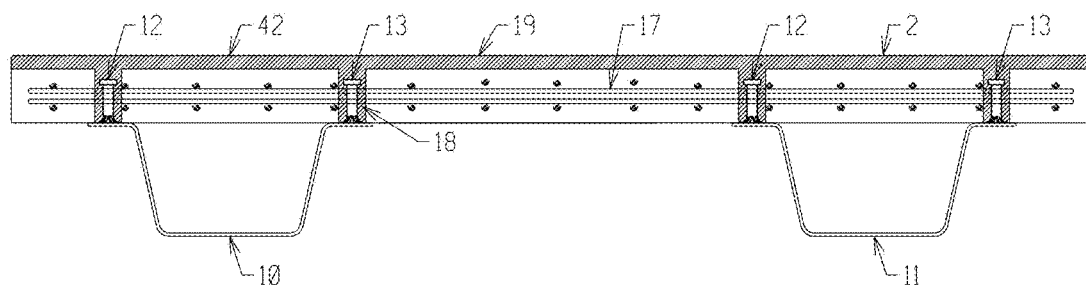
SECTION B-B FIGURE 6C
