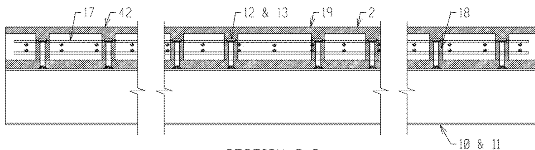
SECTION C-C FIGURE 6B
