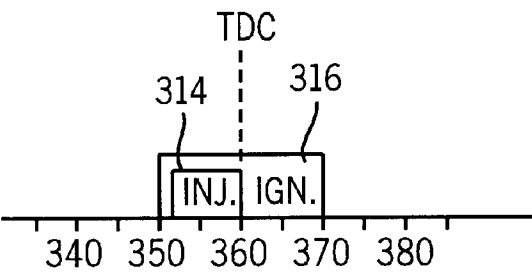
FIG. 8 CRANKSHAFT ANGLE (DEGREES)
