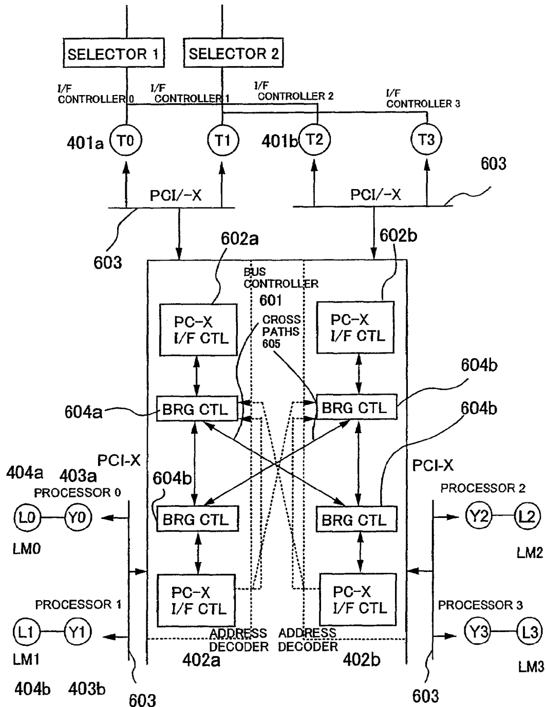
PCI-X SECTION HARDWARE CONFIGURATION
