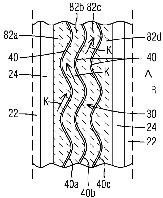
FIG 4B View IV-IV
