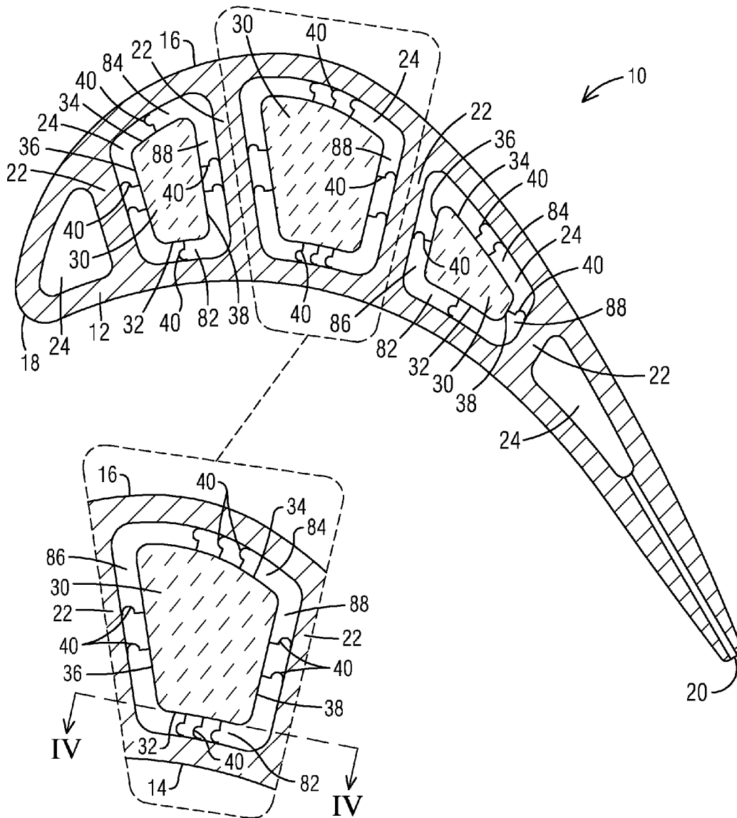
FIG 3 View III-III
