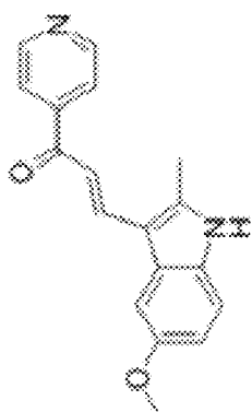
MOMIPP, MW 292.33184
