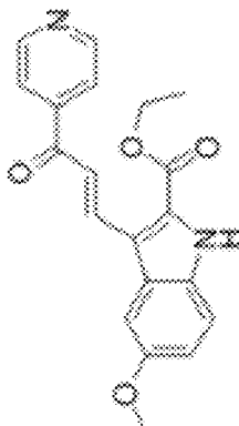
MOCCAEIIP, MW 350.37125
