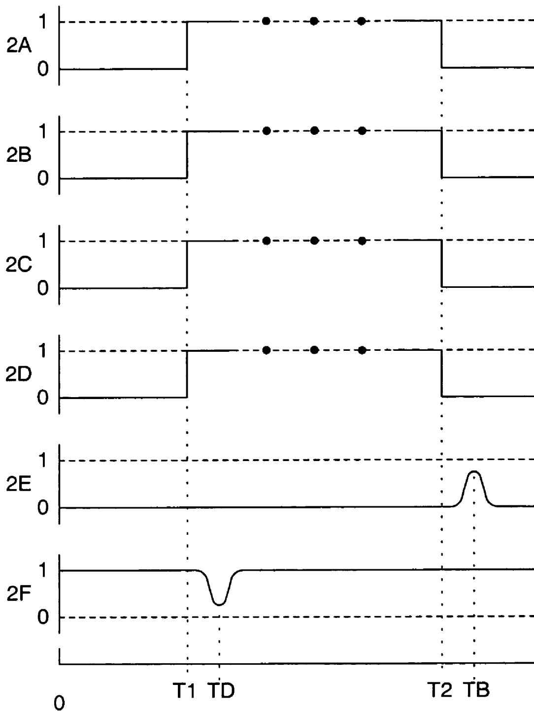
FIG. 2 (CONVENTIONAL)
