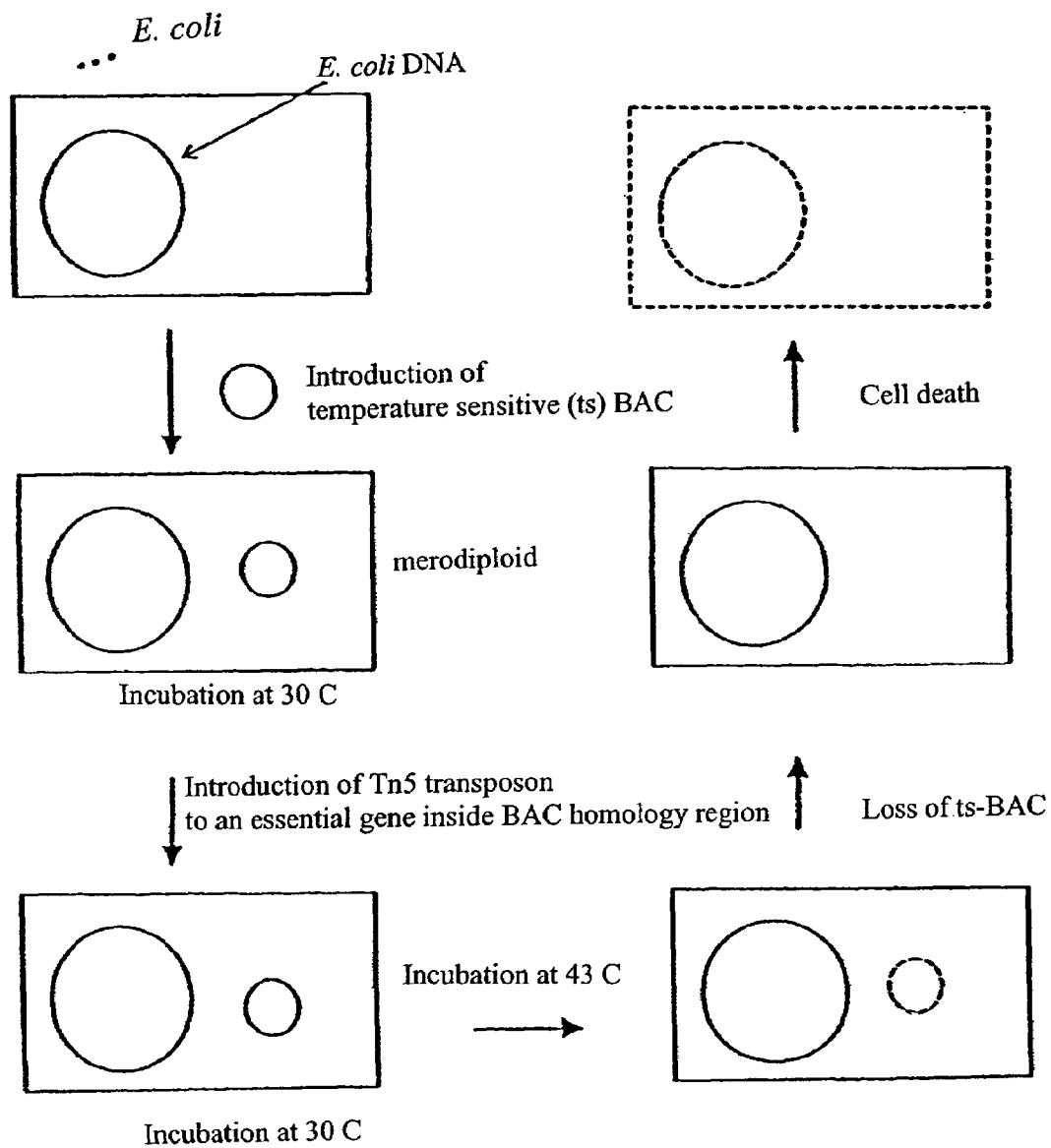
Fig. 1. Diagram of the introduction and the elimination of Tn5 transposon and BACTs in E. coli
