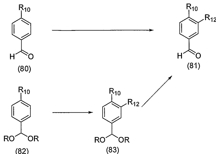
Scheme 12
