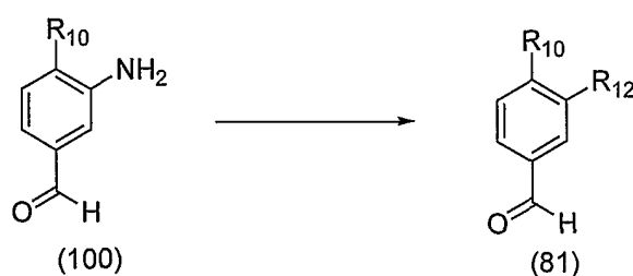
Scheme 19
