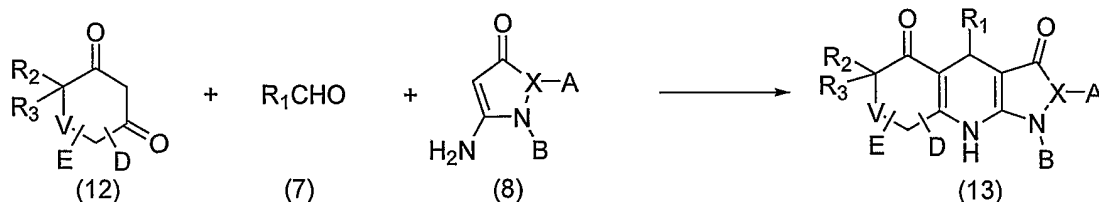
Scheme 5
