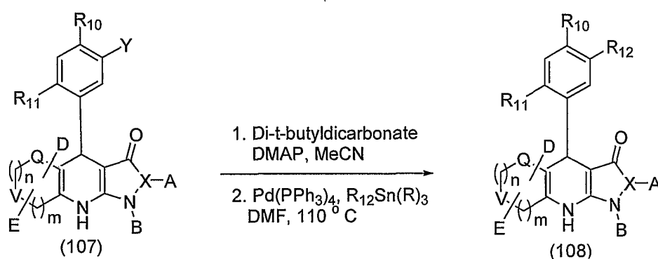
Scheme 23
