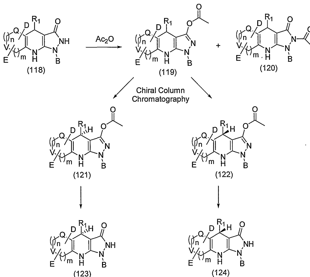
Scheme 27
