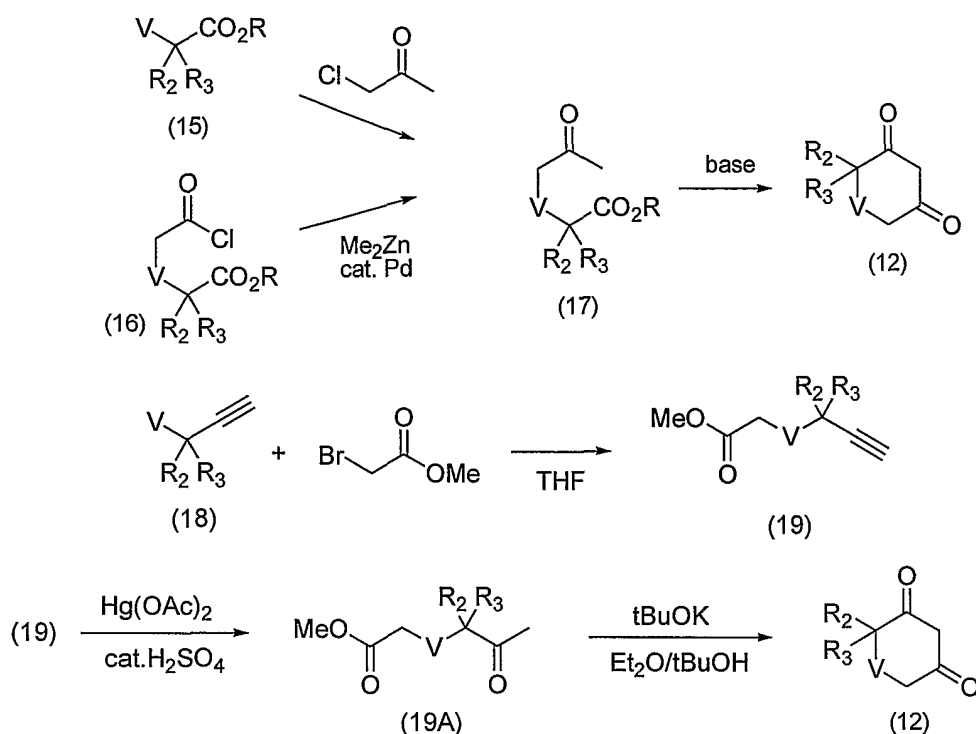
Scheme 6
