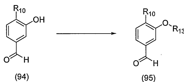
Scheme 17
