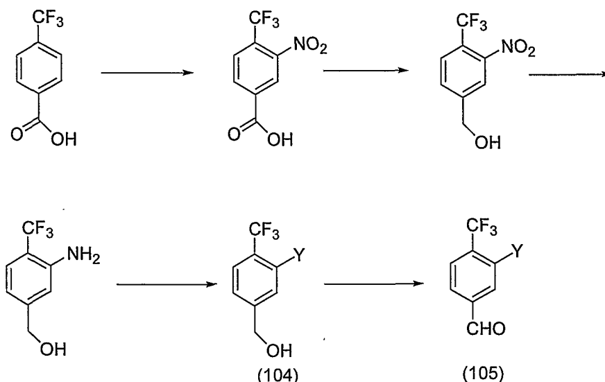
Scheme 22
