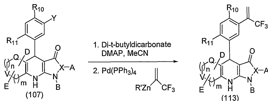
Scheme 25
