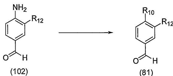
Scheme 20
