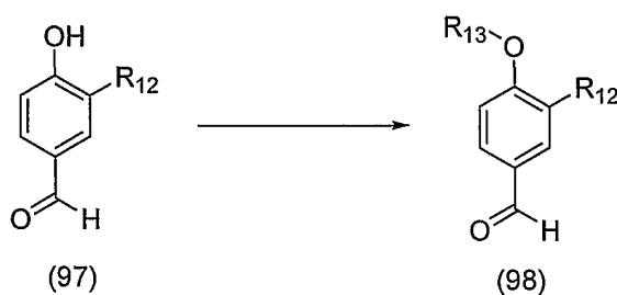
Scheme 18
