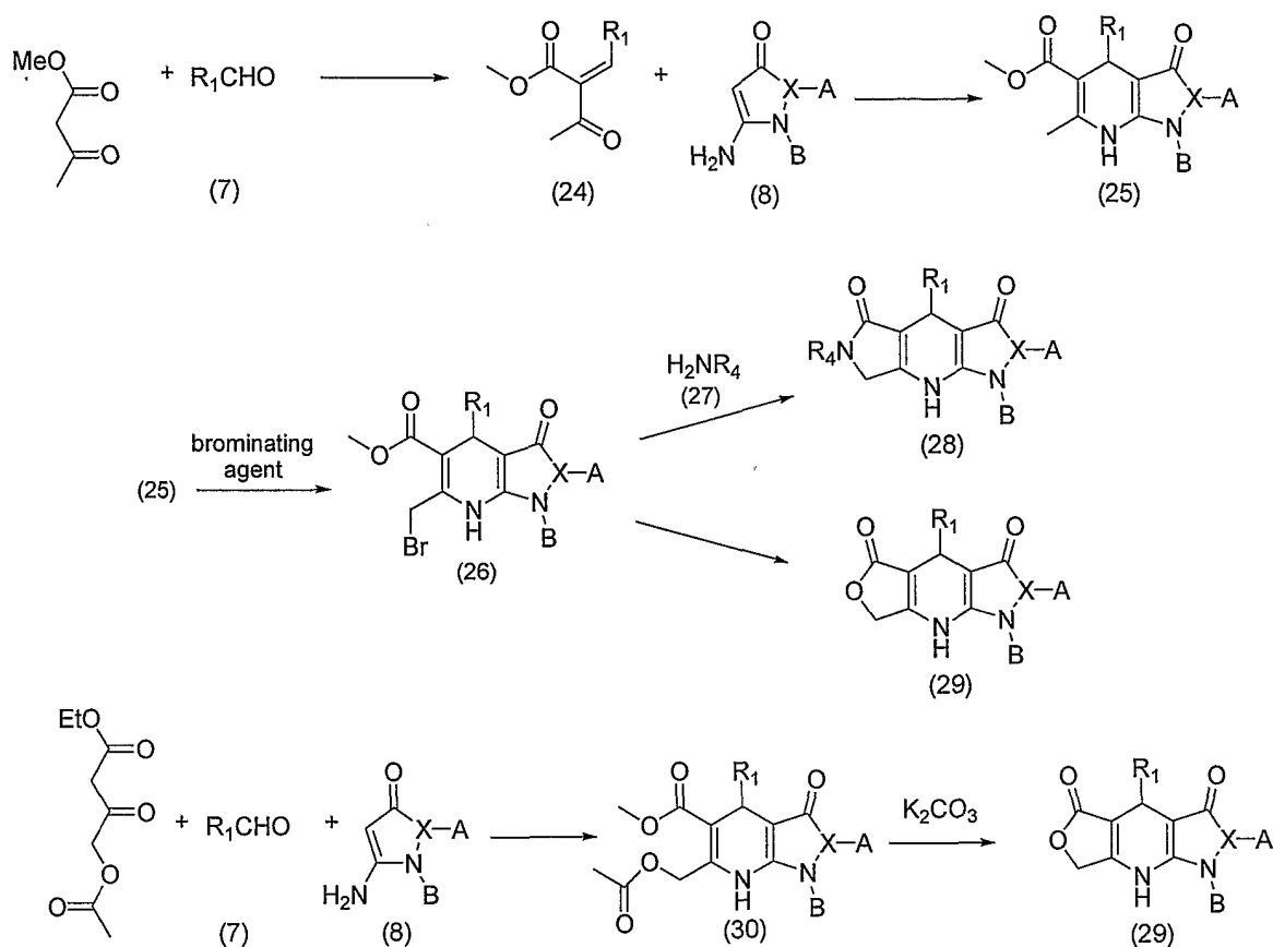
Scheme 8
