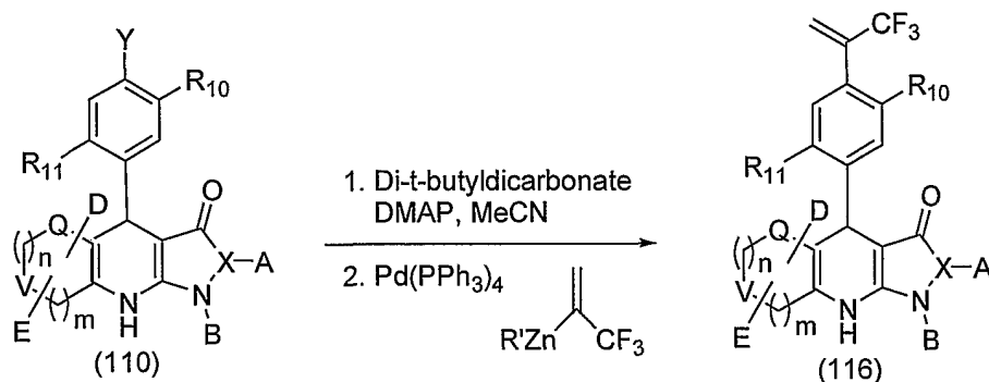
Scheme 26
