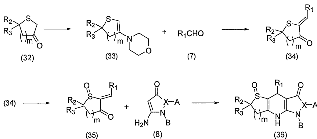
Scheme 9
