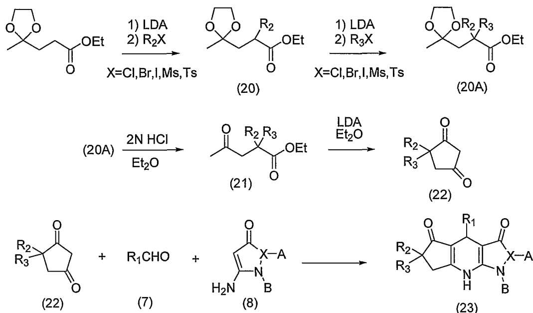
Scheme 7
