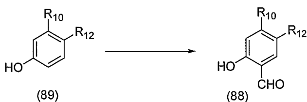
Scheme 14
