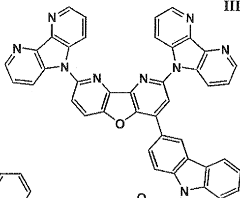
III-50
