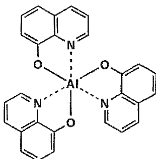
Host-50
