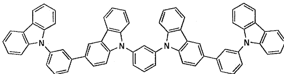
Host-36
