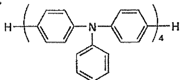
HT-9 (F8-TFB)
