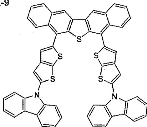
I-9
