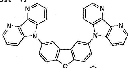
Host-19
