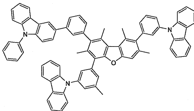
III-24
