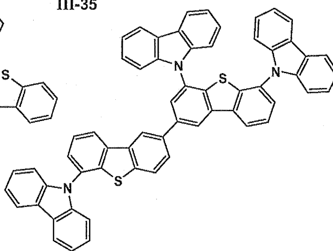
III-35
