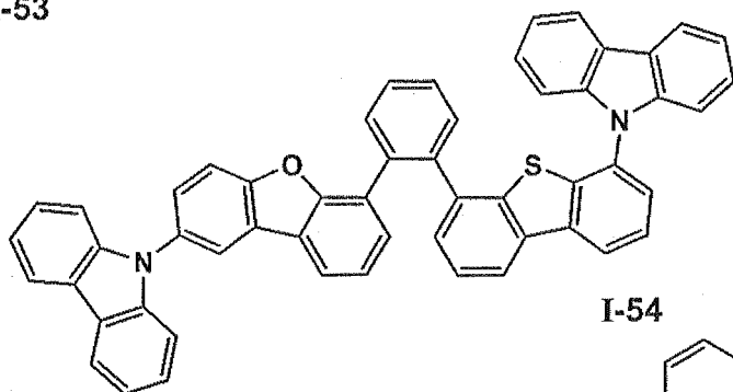
I-53
