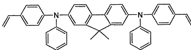
Hole transport compound 6
