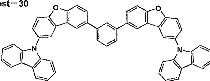
Host-30
