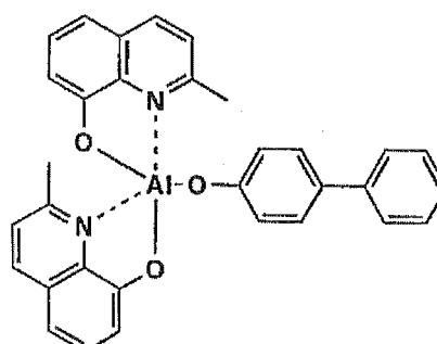
Host-51
