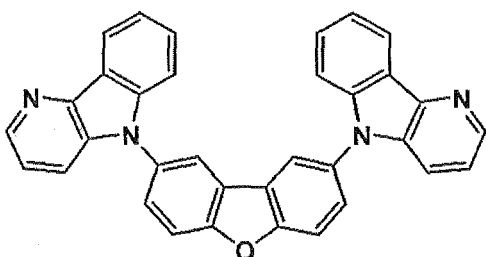
Comparative compound 5
