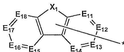
Formula (2A')
