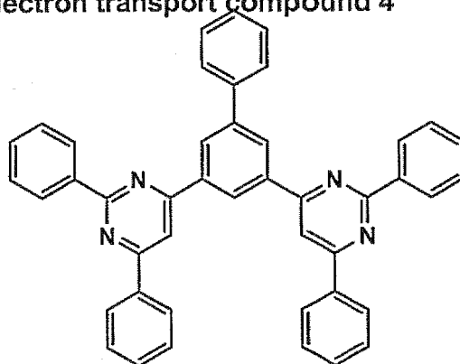
Electron transport compound 4
