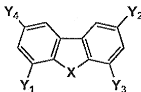
Formula (2)
