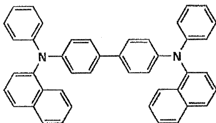
Host-1
