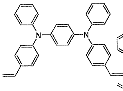
Hole transport compound 4
