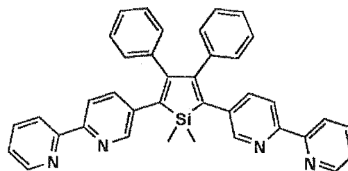
Host-47
