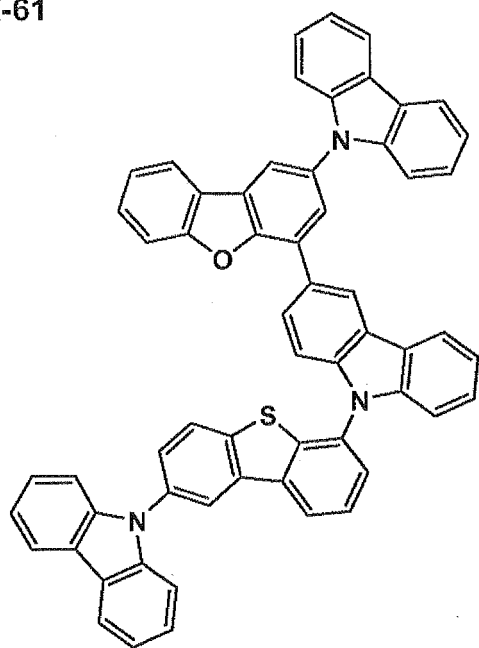
I-61
