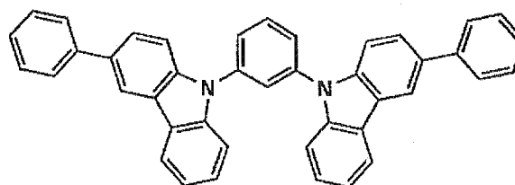
Host-14
