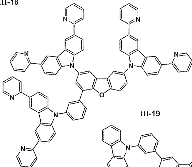
III-18
