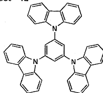
Host-14
