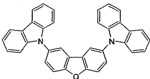
Comparative compound 3
