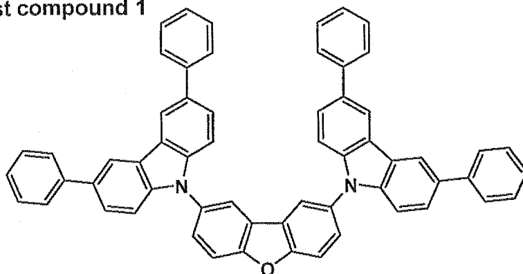
Host compound 1
