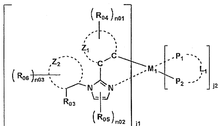
Formula (5)
