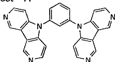
Host-13
