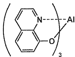
Electron transport compound 5
