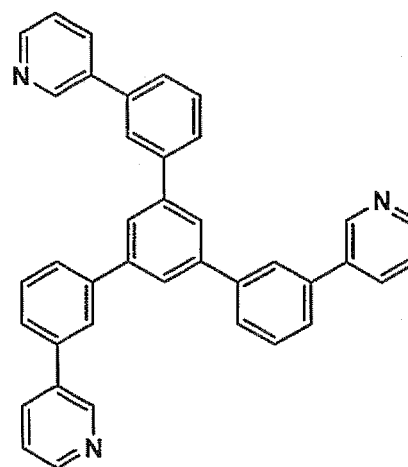
Electron transport compound 2
