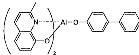
Electron transport compound 6
