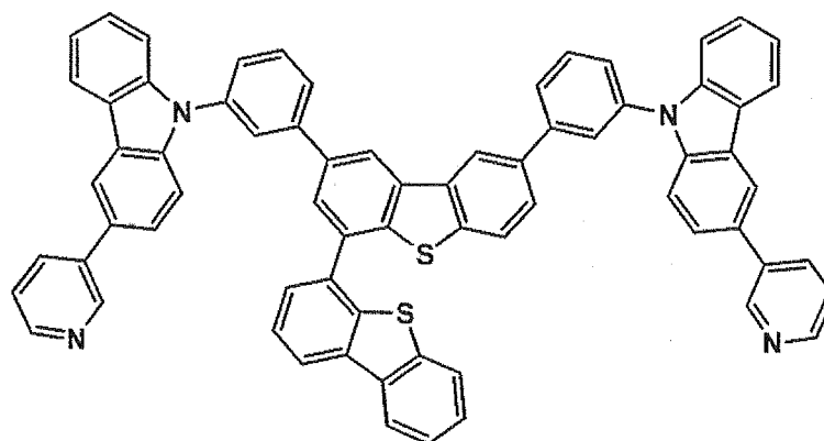
III-19
