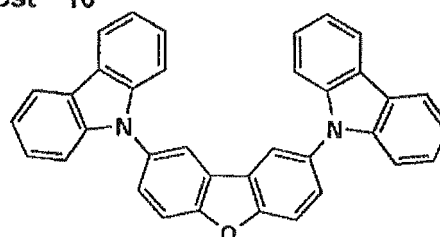
Host-16
