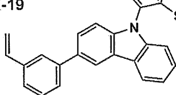
I-21
