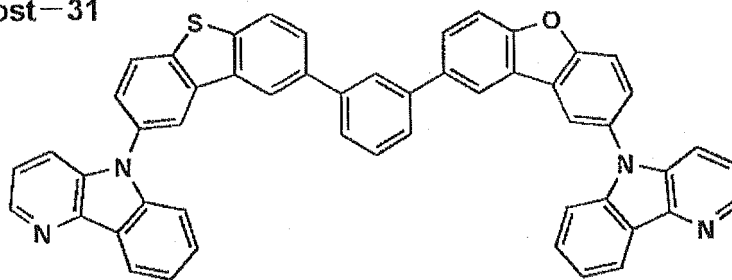
Host-31
