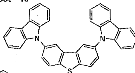
Host-18
