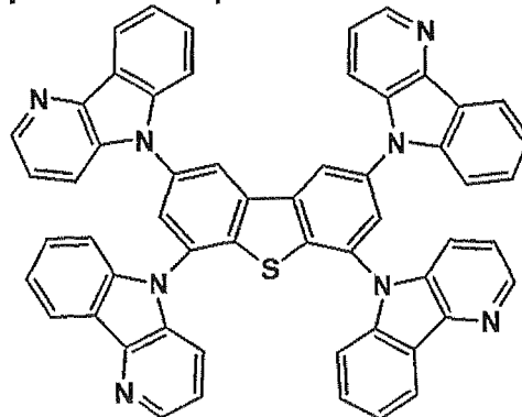
Comparative compound 7
