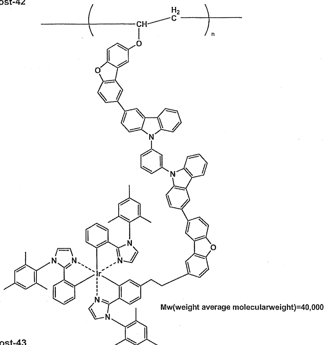
Host-42
