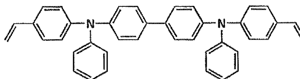
HT-25
