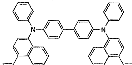
HT-29
