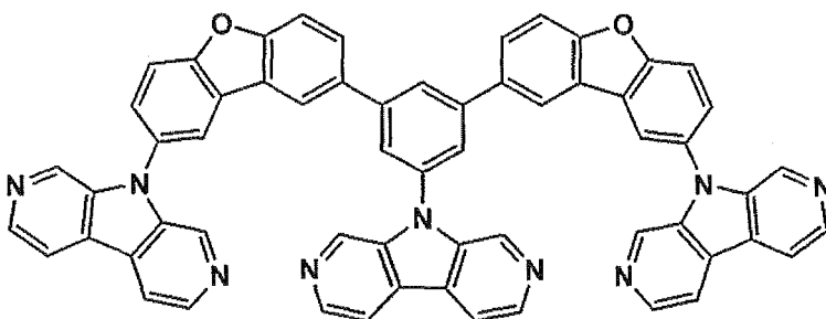
Comparative compound 5
