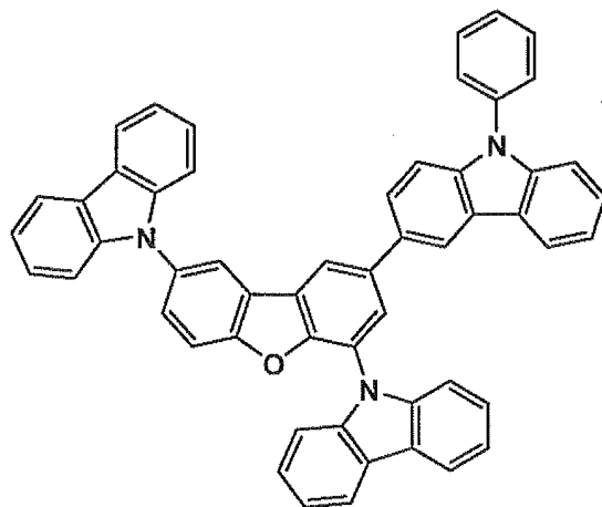
III-5
