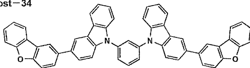
Host-34
