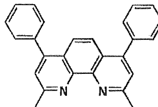
Host-45
