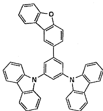
Host-13
