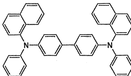
Hole transport compound 1
