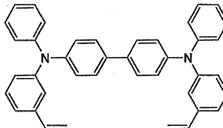
Hole transport compound 3
