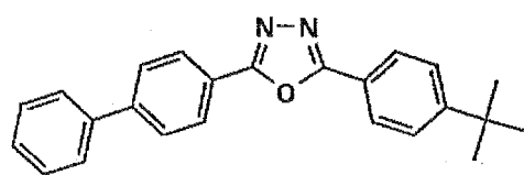
Host-46
