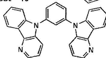
Host-10
