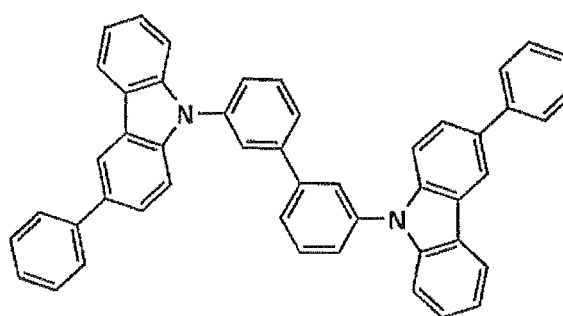
Host-6
