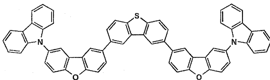
Host-37
