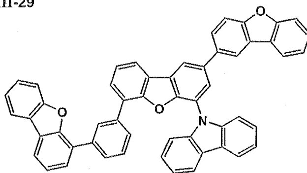
III-29
