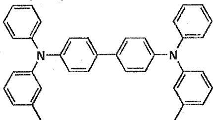
HT-1 (TPD)
