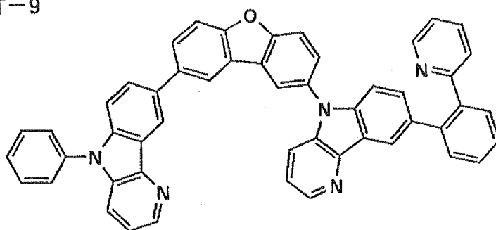
ET-9
