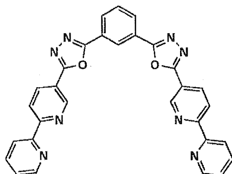
Host-48
