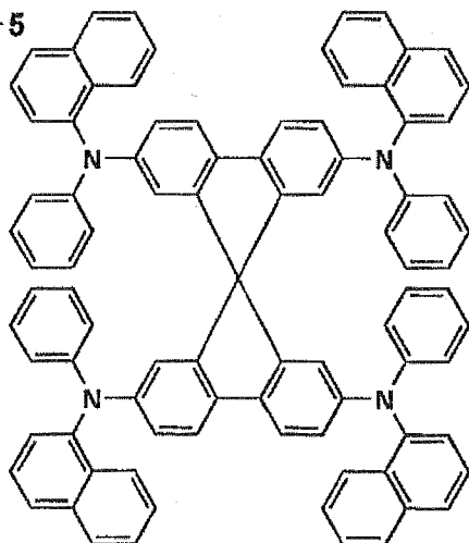
HT-6
