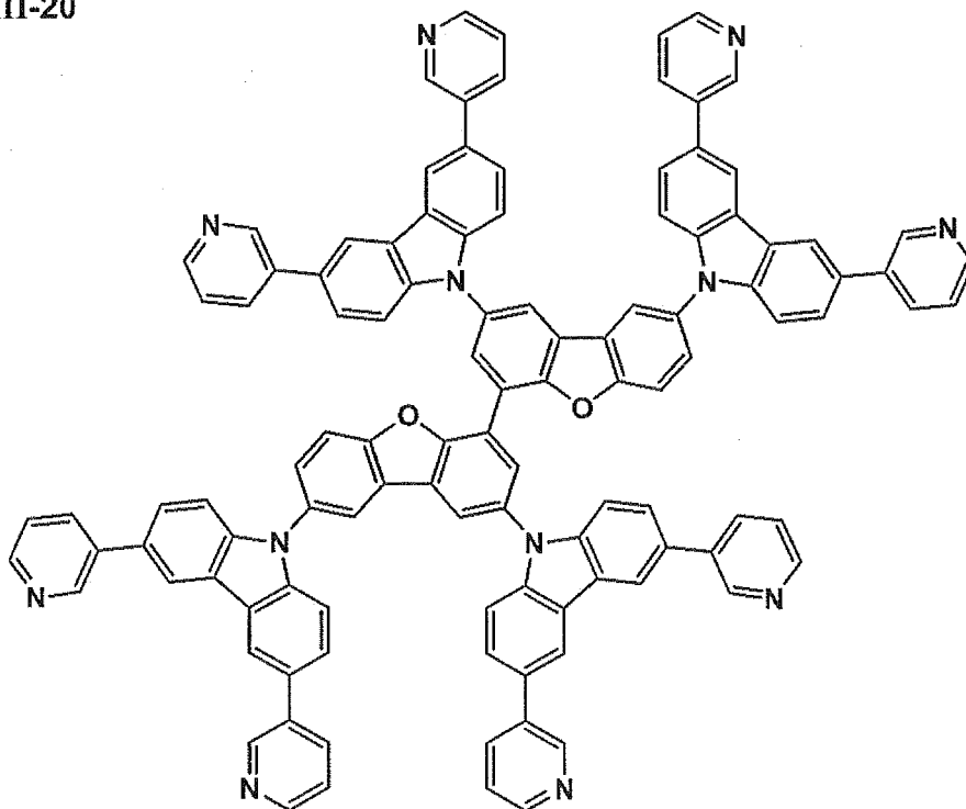
III-20
