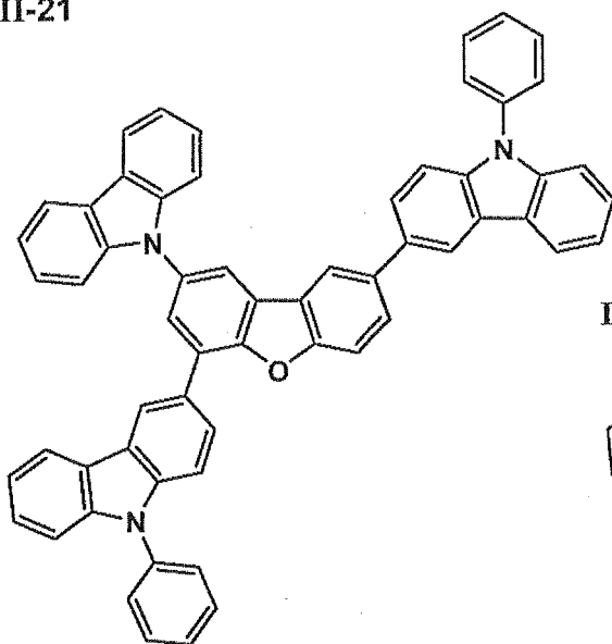
III-21
