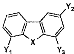
Formula (1)
