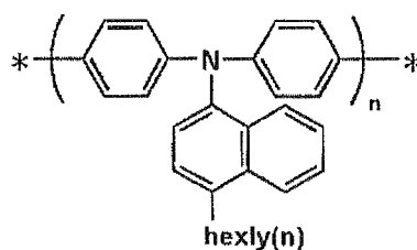
HT-21
