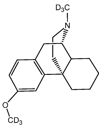
d6-dextromethorphan
