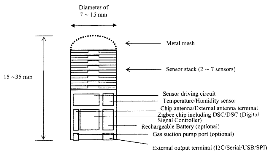
FIG.9 Schematic Diagram of Smart Gas Sensor Capsule
