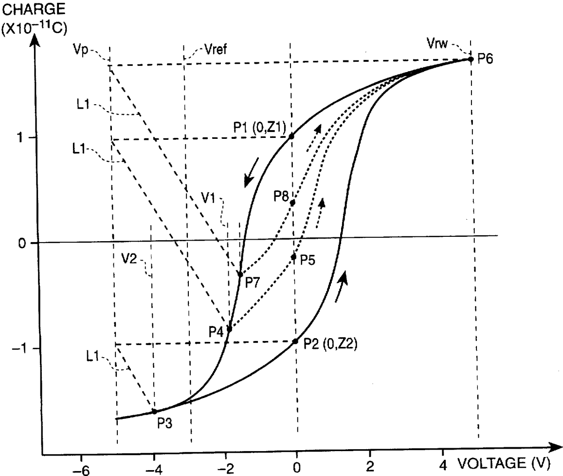
FIG. 20 (PRIOR ART)
