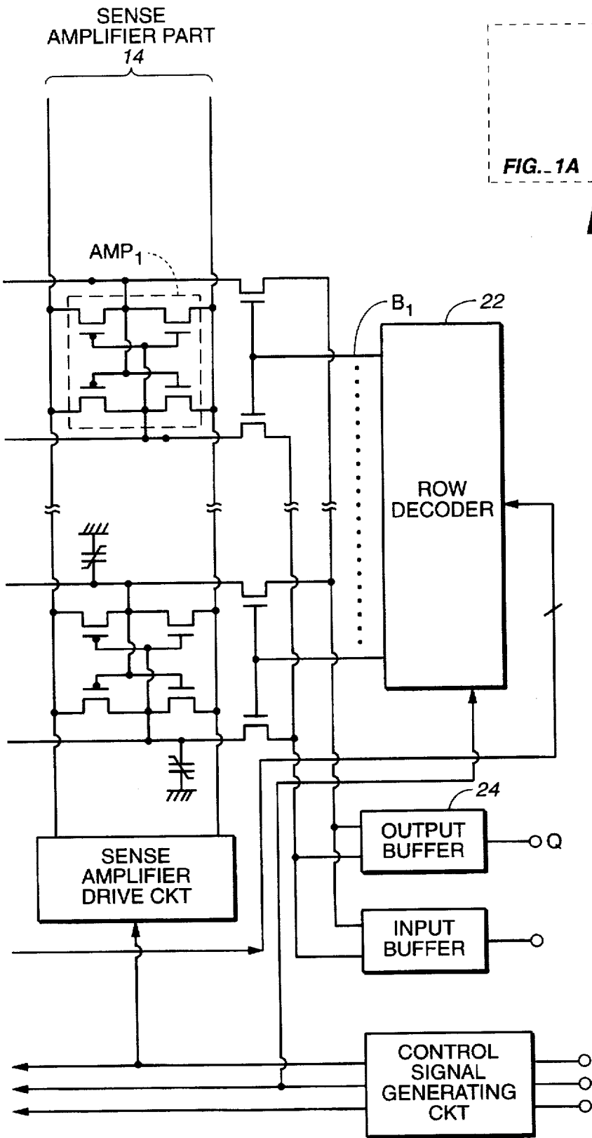
FIG._1C
